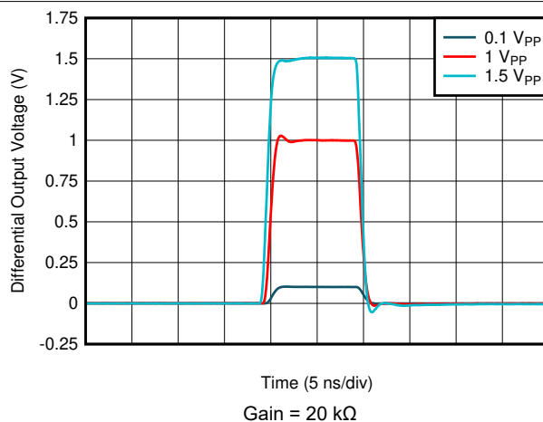
6-20. Pulse Response vs Output Swing
