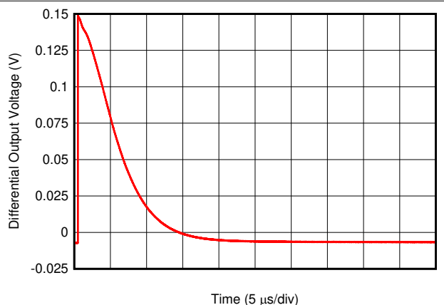
6-25. Turn-Off Time
