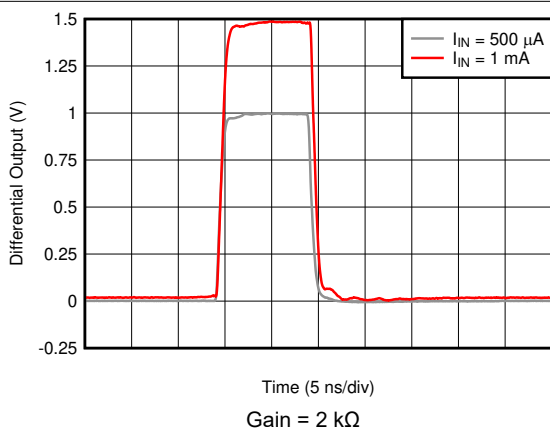
6-21. Overloaded Pulse Response
