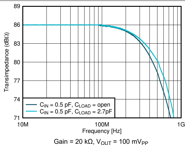
FIG 6-6. Small-Signal Response vs Load Capacitance
