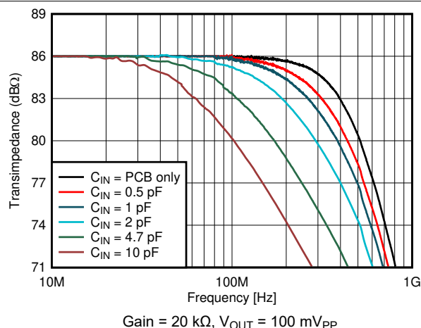
FIG 6-2. Small-Signal Response vs Input Capacitance
