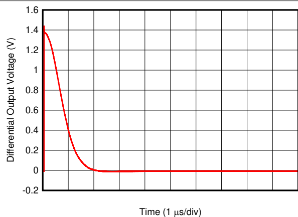
FIG 6-29. Ambient Loop-Cancellation Settling Time
