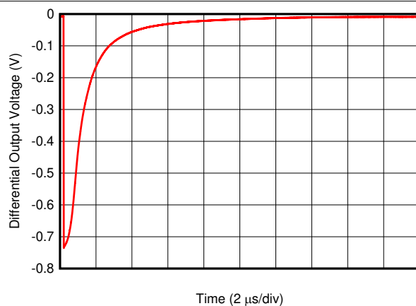
FIG 6-30. Ambient Loop-Cancellation Settling Time
