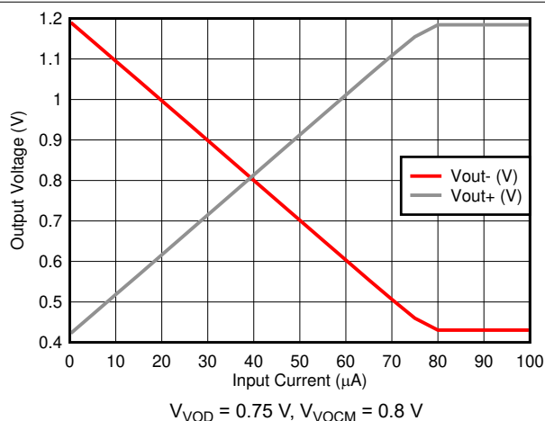
FIG 6-40. Low-side Swing vs Input Current
