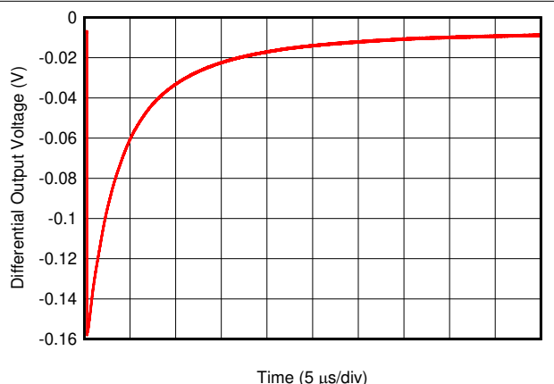
6-26. Turn-Off Time
