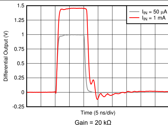
6-22. Overloaded Pulse Response
