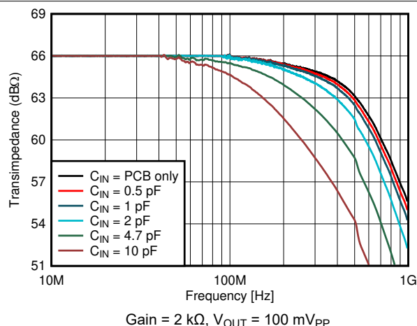
FIG 6-1. Small-Signal Response vs Input Capacitance
