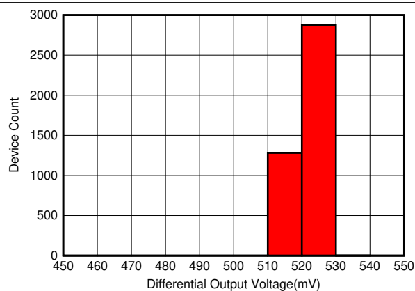
FIG 6-48. Differential Output Offset Voltage ( V_{OD} ) Distribution
