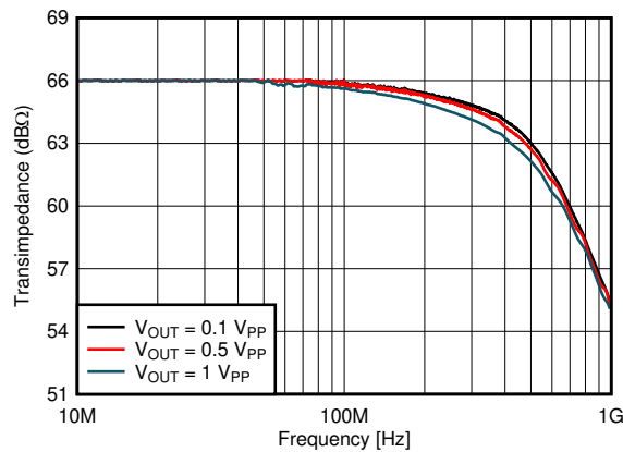
Figure 8-4. Bandwidth vs Output Swing (Gain = 2 kΩ)
