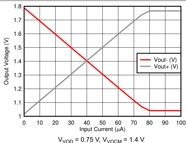
FIG 6-39. High-side Swing vs Input Current
