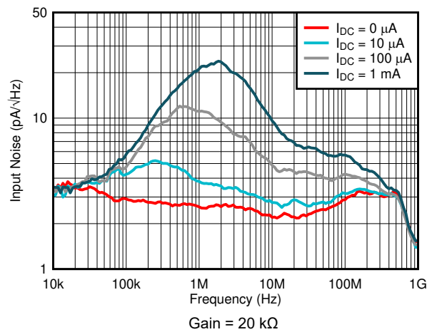
6-16. Input Noise Density vs Ambient-Light DC Current
