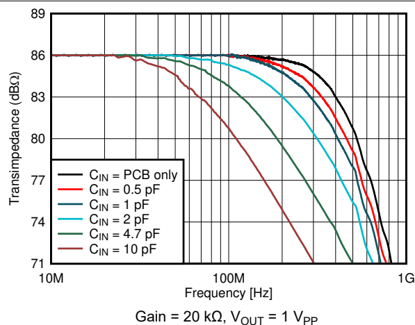
FIG 6-4. Large-Signal Response vs Input Capacitance
