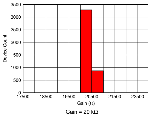
6-46. Transimpedance Gain (High) Distribution
