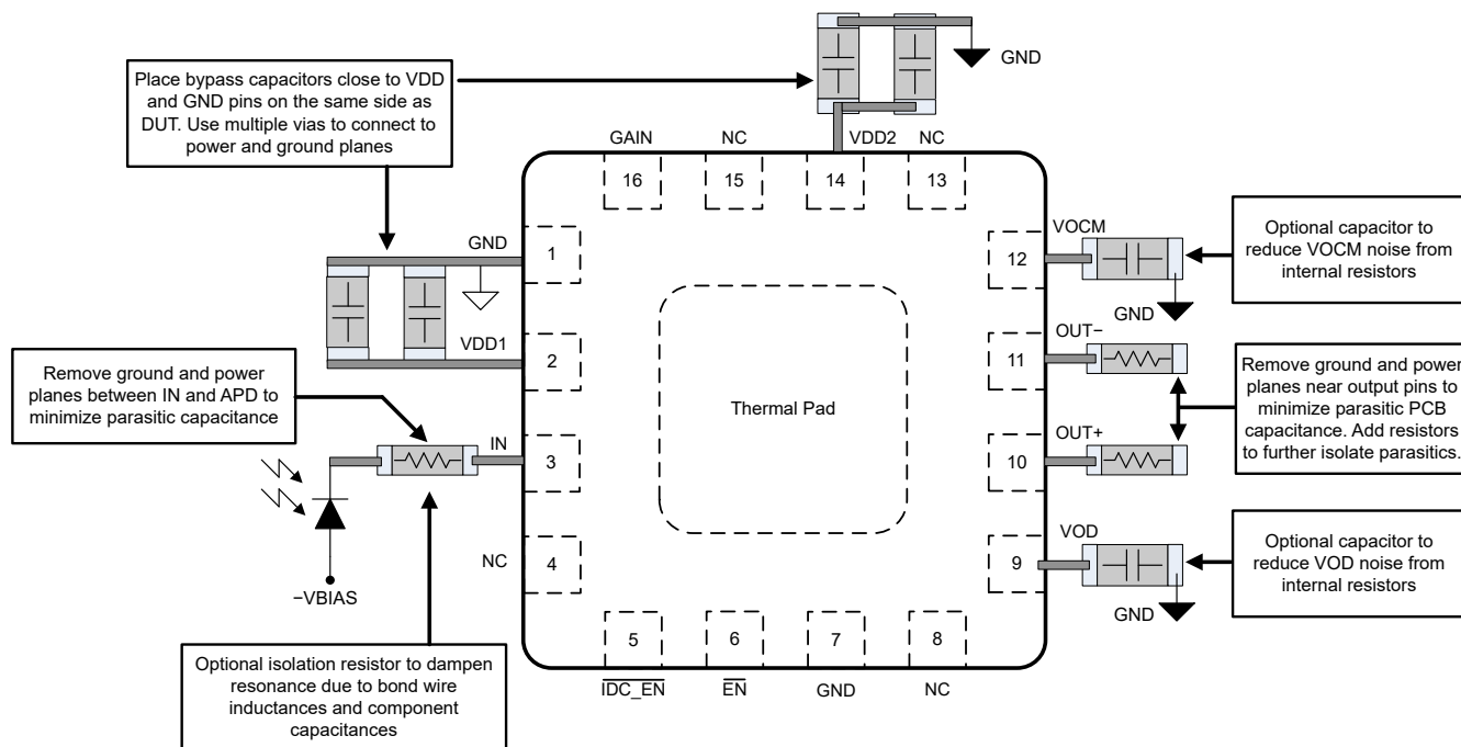
8-8. Layout Recommendation
