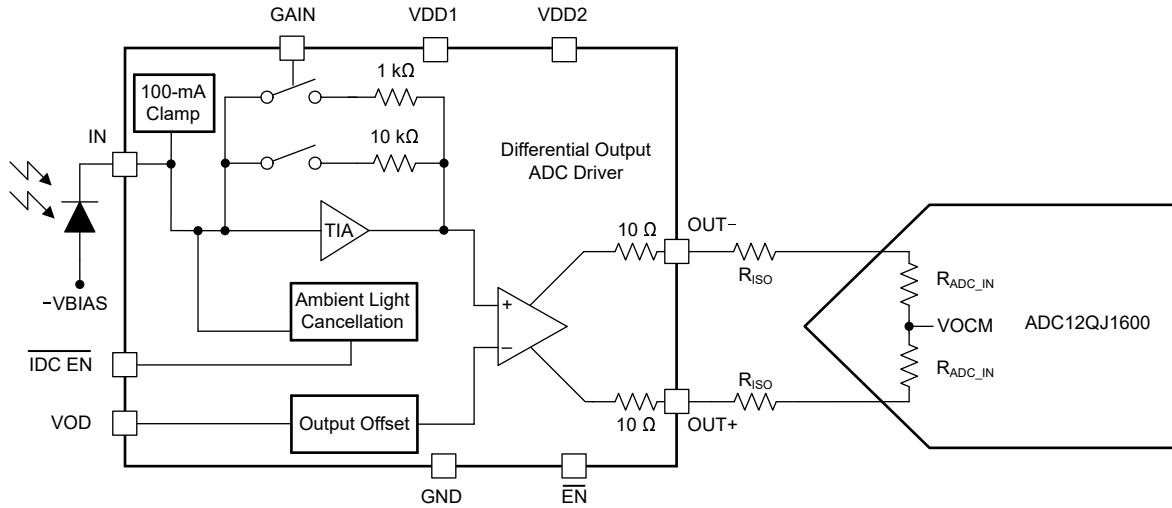
図 8-2. LMH32401-Q1 to ADC Interface With a Matching Resistor Network
