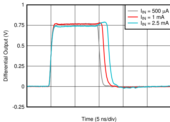
Figure 8-6. Pulse Response vs Input Current (Gain = 2 kΩ)
