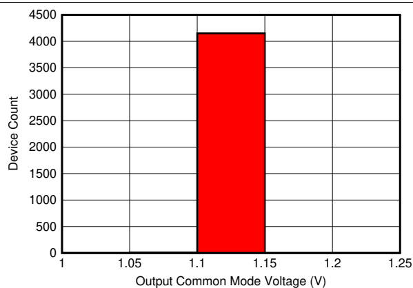
FIG 6-47. Output Common-Mode Voltage ( V_{OCM} ) Distribution
