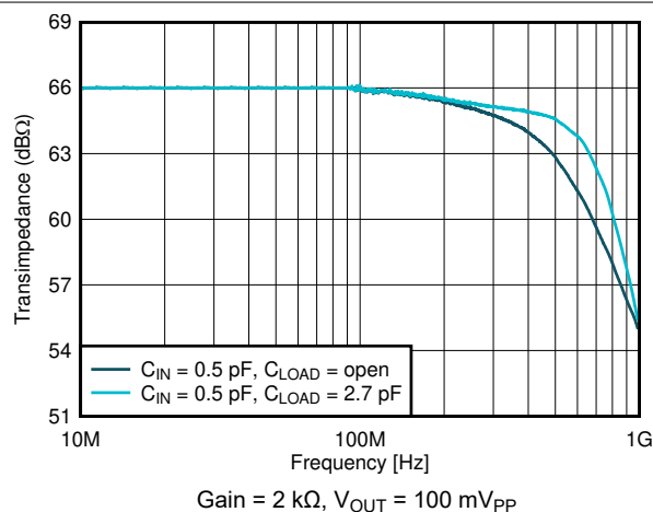
FIG 6-5. Small-Signal Response vs Load Capacitance
