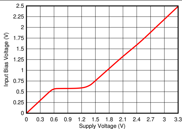
FIG 6-35. Input Bias Voltage vs Supply Voltage
