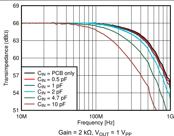
FIG 6-3. Large-Signal Response vs Input Capacitance
