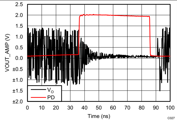
Figure 32. Power Down Timing
