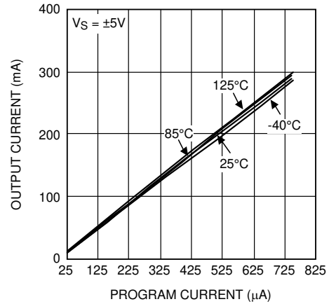
FIG 5-32. Output Short Circuit Current — Sourcing vs. Program Current
