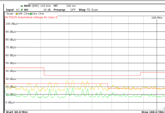
V_{IN} = 12.5V V_{OUT} = 3.3V F_{sw} = 2.2MHz 負荷 = 3A
