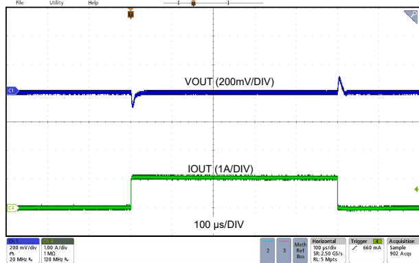
LMQ66430MC3 V_{OUT} = 3.3V 2.2MHz (FPWM) 0A ~ 1A, 1A/ \mu s 固定
