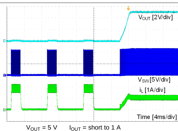
Figure 29. Short Recovery
