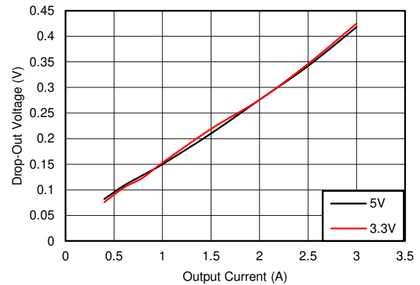
8-10. Typical Dropout Voltage vs Output Current in Frequency Foldback f_{SW} = 140\text{ kHz}
