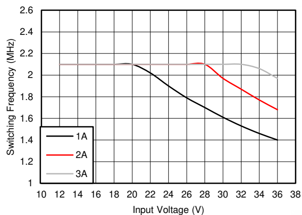
8-13. Switching Frequency vs Input Voltage V_{OUT} = 3.3\text{ V}
