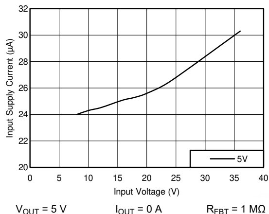
Figure 9-10. Input Supply Current
