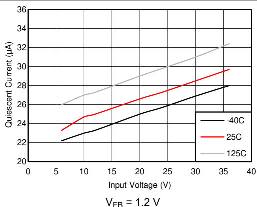
7-1. Non-Switching Input Supply Current
