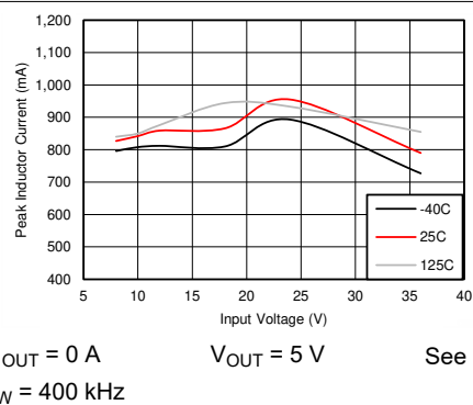
7-6. I_{PEAK-MIN}
