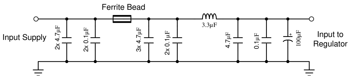
Figure 9-28. Typical Input EMI Filter Filter Used Only for EMI Measurements Found in Application Curves
