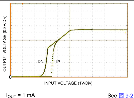
7-5. UVLO Thresholds
