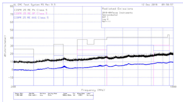
9-24. Radiated EMI Log-Periodic Antenna (Horizontal)
