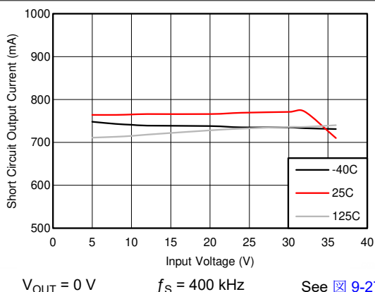
7-3. Short-Circuit Output Current
