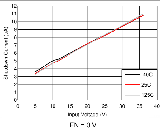
7-2. Shutdown Supply Current
