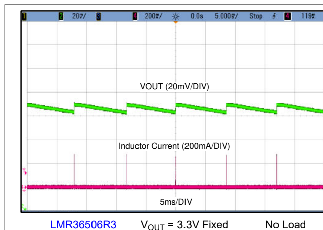
9-16. Output Ripple
