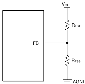
図 8-6. Setting Output Voltage for Adjustable Output Variant
