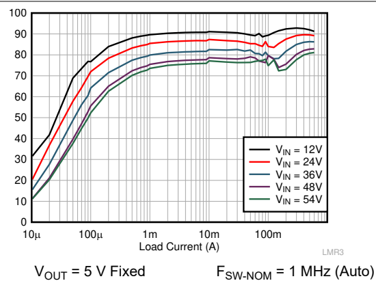
7-4. Efficiency 5-V Output, Auto Mode
