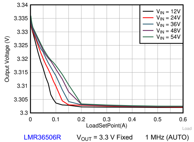
图 9-5. Line and Load Regulation
