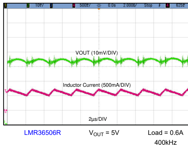
9-17. Output Ripple
