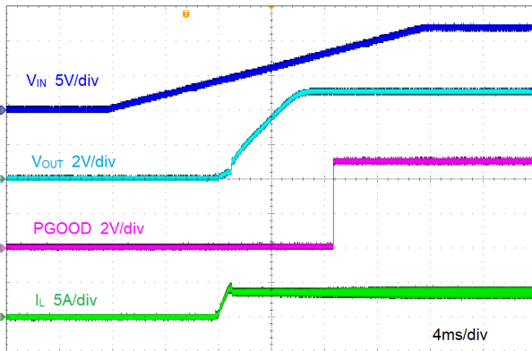
8-4. Start-Up by V_{IN}
