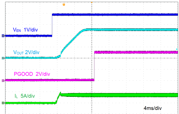
8-5. Start-Up by EN
