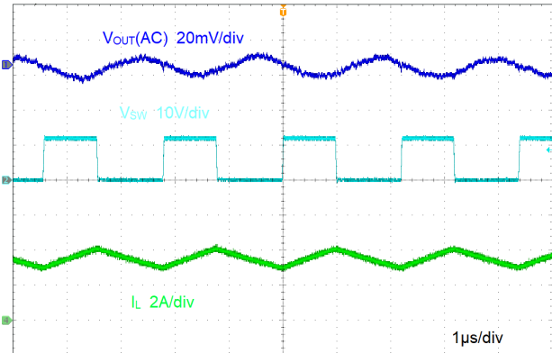
8-3. Ripple at Full Load
