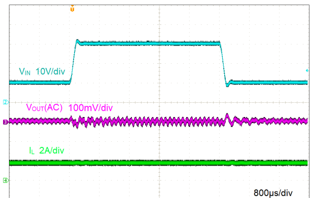
8-7. Line Transient
