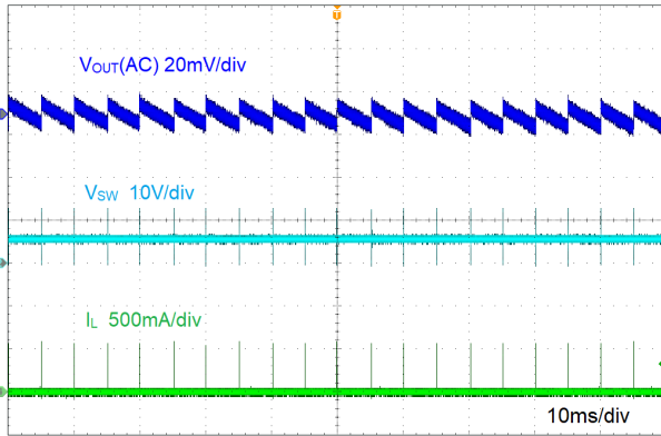
8-2. Ripple at No Load
