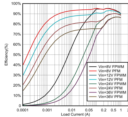
図 6-4. 5-V Efficiency Versus Load Current
