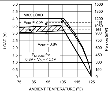
Figure 8. Current Derating
