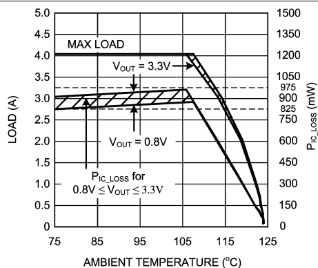
Figure 7. Current Derating
