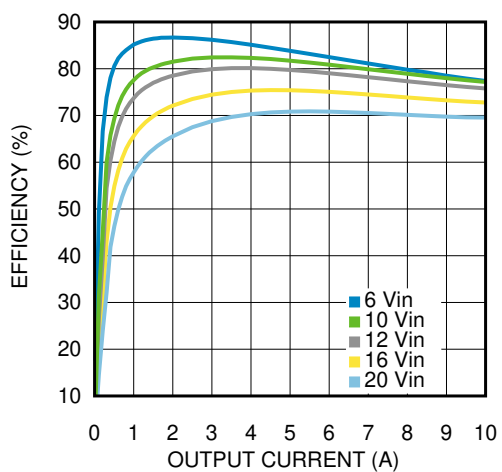
FIG 6-23. Efficiency 1.5-V Output at 85°C
