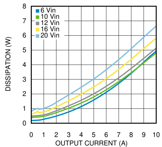
FIG 6-18. Dissipation 3.3-V Output at 85°C
