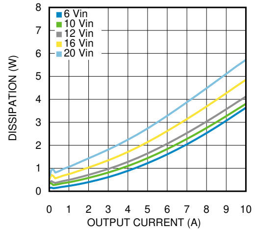
FIG 6-14. Dissipation 1-V Output at 25°C
