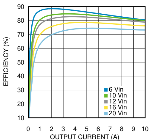
FIG 6-21. Efficiency 1.8-V Output at 85°C
