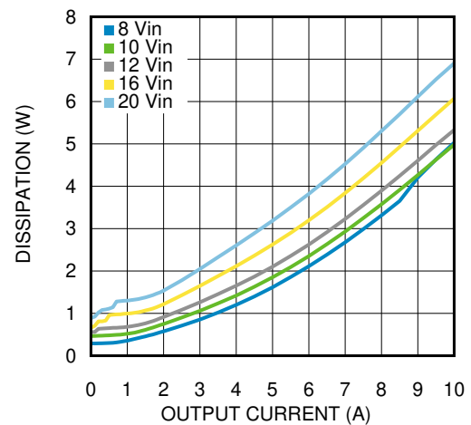
FIG 6-16. Dissipation 5-V Output at 85°C
