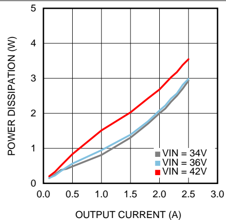
Figure 24. Power Dissipation V_{OUT} = 30\text{ V} , T_A = 85^\circ\text{C}
