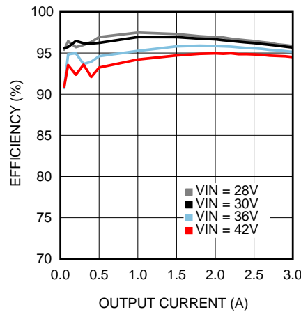
Figure 47. Efficiency V OUT = 24 V, T A = 25°C
