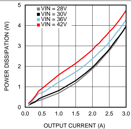
Figure 22. Power Dissipation V_{OUT} = 24\text{ V} , T_A = 85^\circ\text{C}
