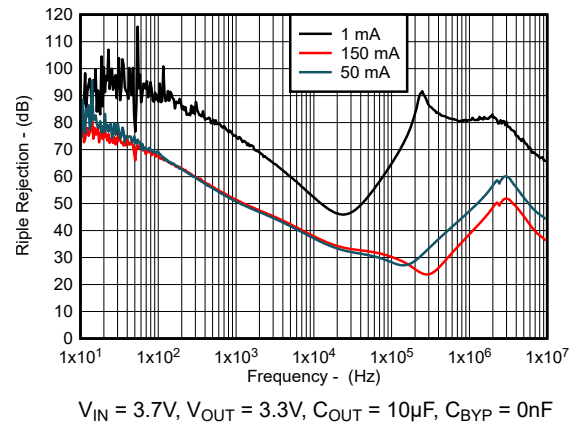
図 5-14. Ripple Rejection vs Frequency (New Chip)
