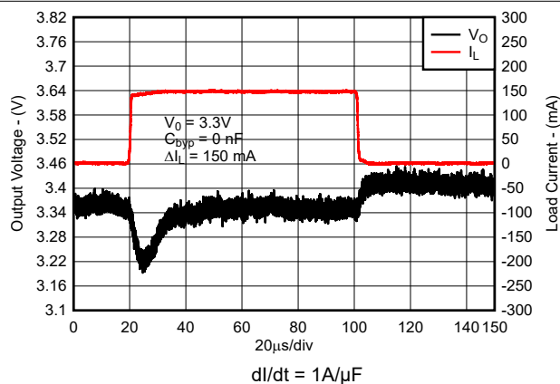
Figure 7-13. Load Transient Response (New Chip)
