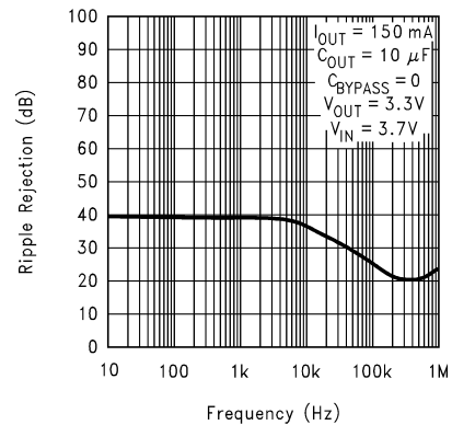
図 5-10. Ripple Rejection vs Frequency (Legacy Chip)
