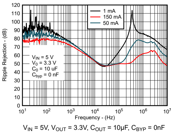
図 5-9. Ripple Rejection vs Frequency (New Chip)
