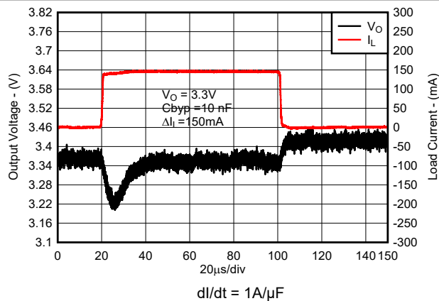
Figure 7-11. Load Transient (New Chip)
