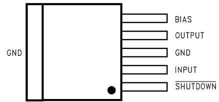
TO-263, Top View
