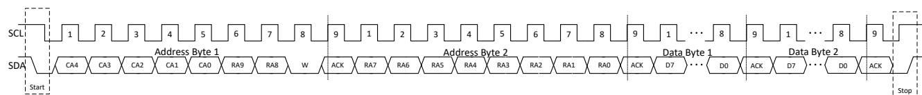
Figure 8-14. I²C Write Timing
