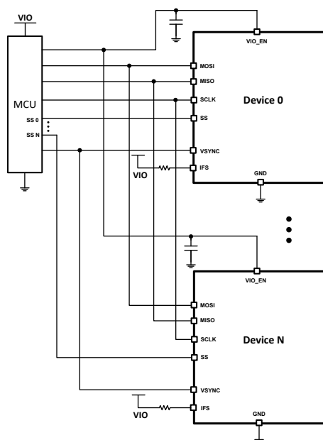
8-19. SPI Multiple Devices Connection
