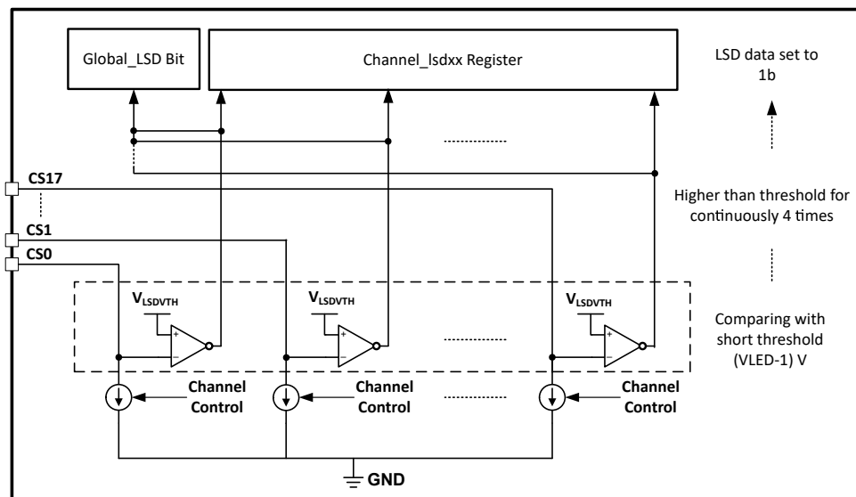
8-12. LSD Circuit
