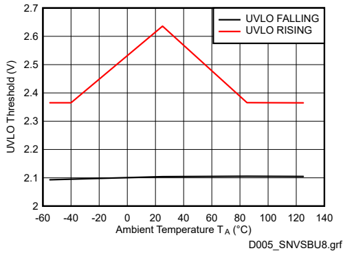
Figure 6-3. V_{CC} UVLO Rising and Falling Thresholds
