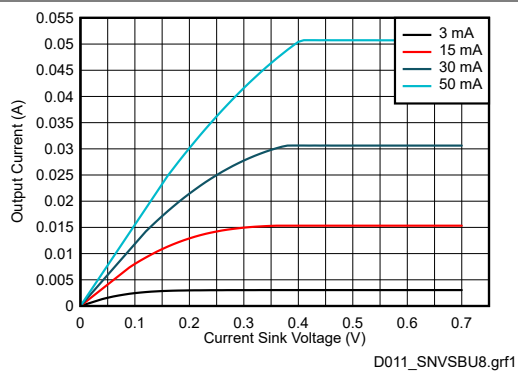
6-9. Current Sinks Voltage vs Current
