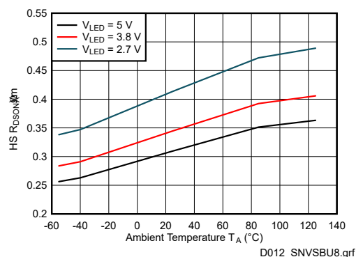
6-10. High Side Switch R_{DS(on)}
