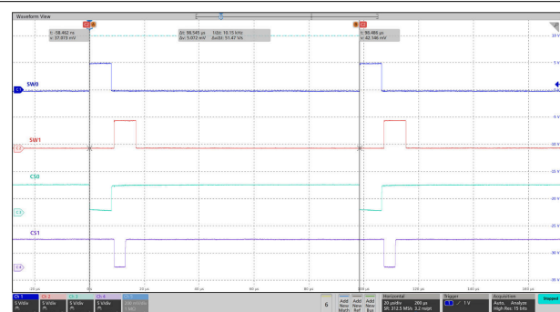
図 9-3. Scan Lines and Current Sinks Waveforms of SW0, SW1, CSR0(CS0), CSG0(CS1)
