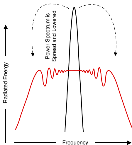
FIG 7-2. Spread-Spectrum Modulation
