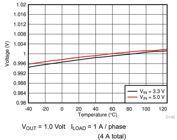
Figure 8-5. Output Voltage vs Temperature
