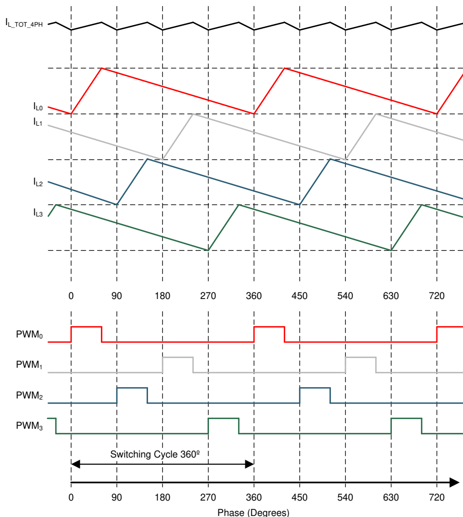
FIG 7-2. Example of PWM Timings, Inductor Current Waveforms, and Total Output Current in 4-Phase Configuration.
