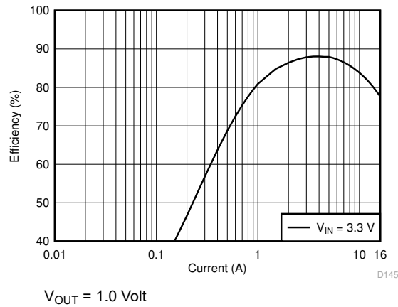
Figure 8-2. Efficiency in Forced-PWM-Four-Phase Mode
