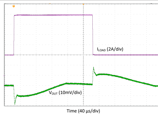
8-11. Transient Load Step Response, Forced-PWM-Four-Phase Mode, T_A = +25^\circ\text{C}
