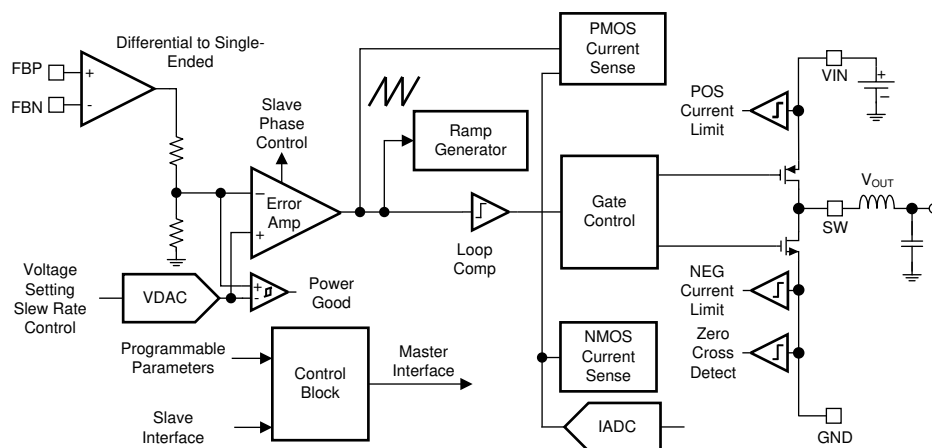
7-1. Detailed Block Diagram Showing One Core
