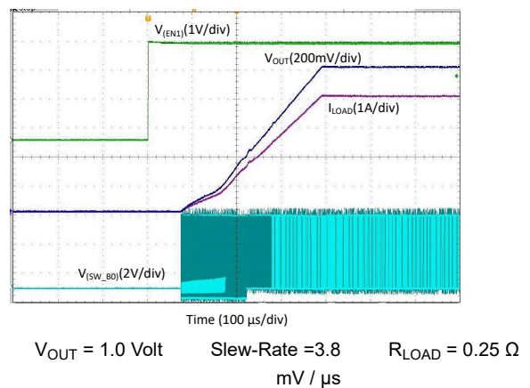
Figure 8-7. Start-Up With EN1, Forced-PWM-Four-Phase Mode
