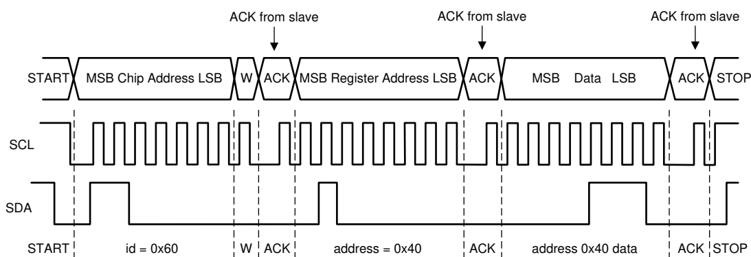
7-15. Write Cycle (w = write; SDA = 0), id = Device Address = 0x60 for LP875761-Q1
