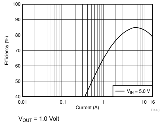
Figure 8-3. Efficiency in Forced-PWM-Four-Phase Mode
