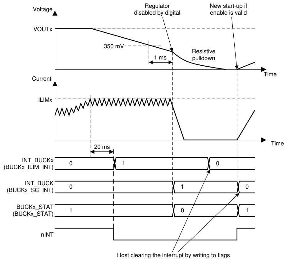
Figure 7-10. Overload Situation
