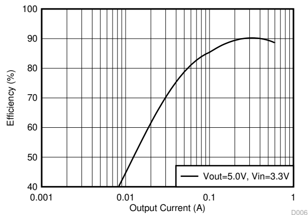
9-21. Boost Efficiency
