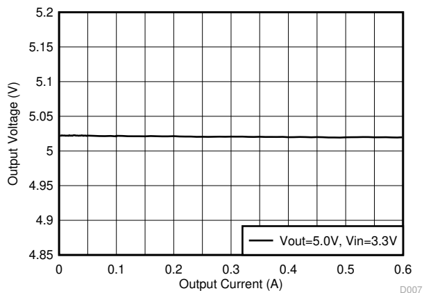
9-22. Boost Output Voltage vs Load Current
