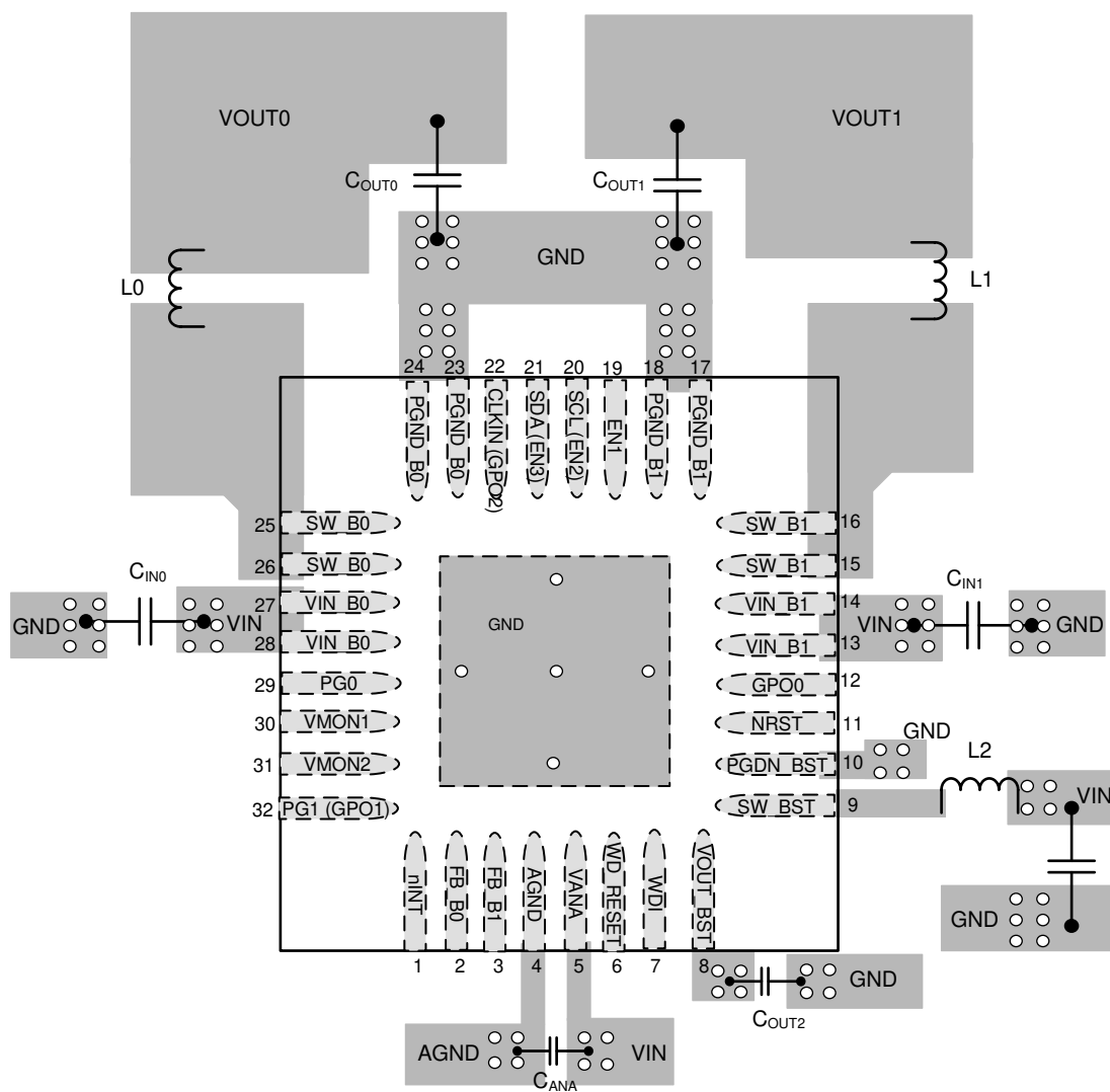
11-1. LP87702-Q1 Board Layout Example
