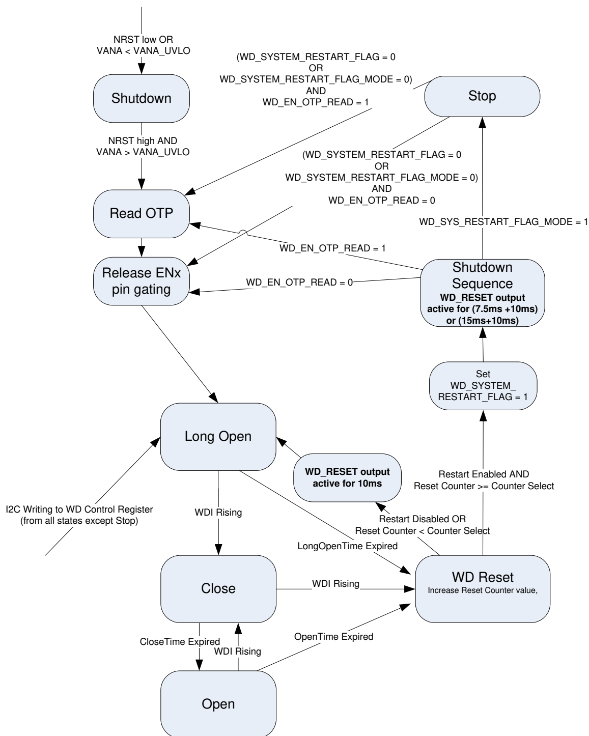
图 8-8. Watchdog Operation
