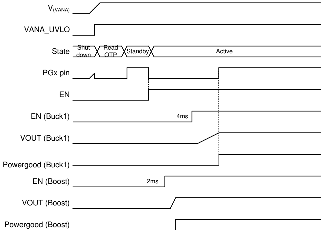
8-11. PGx Pin Operation in Continuous Mode
