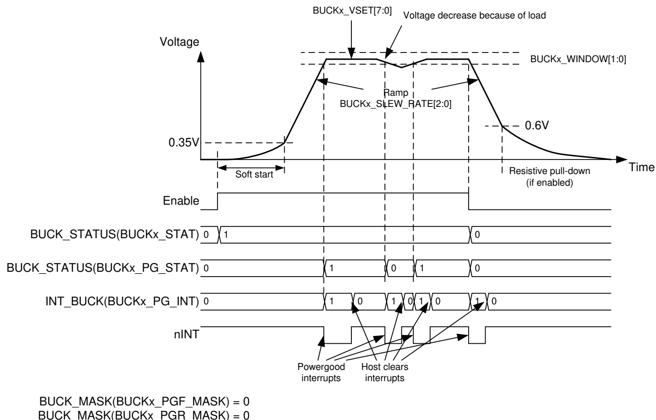
8-4. Buck Converter Enable and Disable
