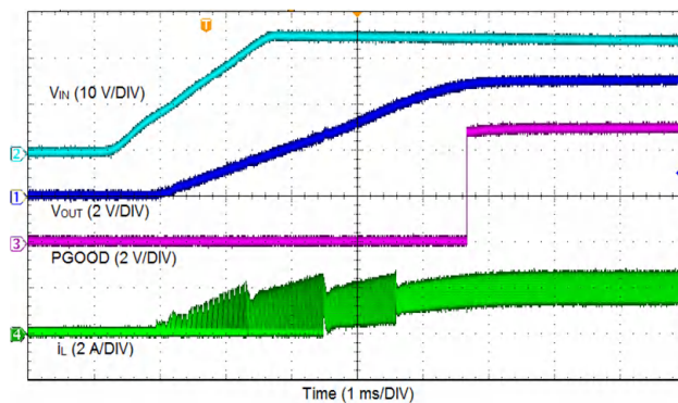
图 9-3. Start-up By V_{IN}
