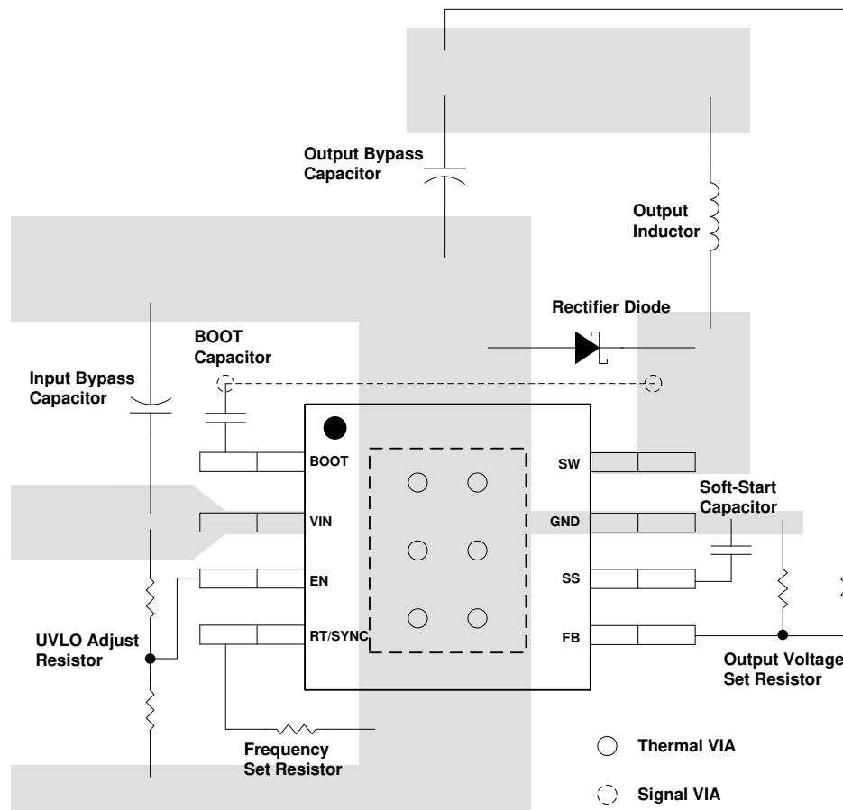
11-1. Layout
