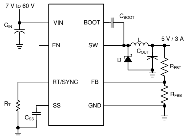
Figure 9-1. Application Circuit, 5-V Output
