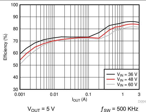
7-4. Efficiency vs Load Current
