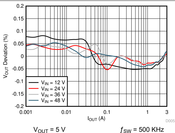
7-5. Load Regulation
