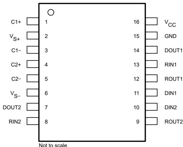
図 4-1. D (SOIC) , DW (SOIC), N (PDIP), or PW (TSSOP) 16-Pin Package (Top View)
