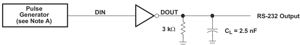
✎ 6-2. Driver Test Circuit and Waveforms for t_{PHL} and t_{PLH} Measurements (5- \mu s Input)
