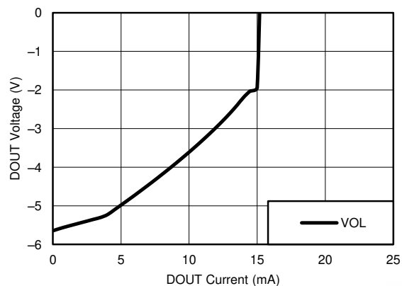
FIG 6-2. DOUT V_{OL} vs Load Current, Both Drivers Loaded
