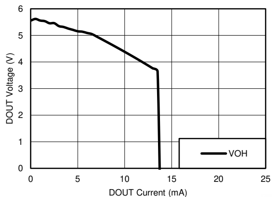
FIG 6-1. DOUT V_{OH} vs Load Current, Both Drivers Loaded
