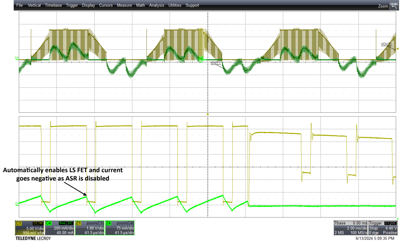
図 9-7. ASR Disabled in Synchronous Modulation
