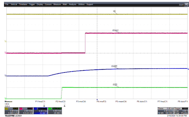
図 9-10. Device Powerup with nSLEEP
