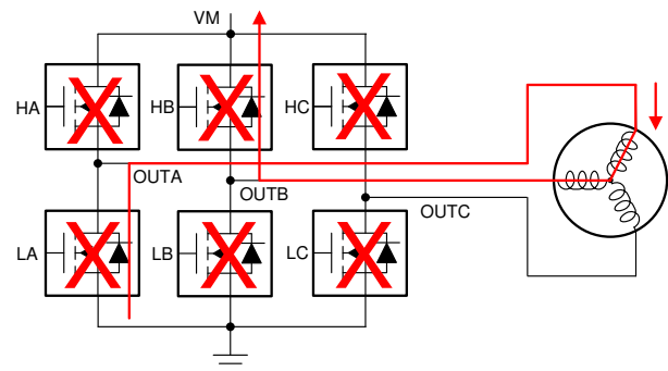
図 7-25. Coast State
