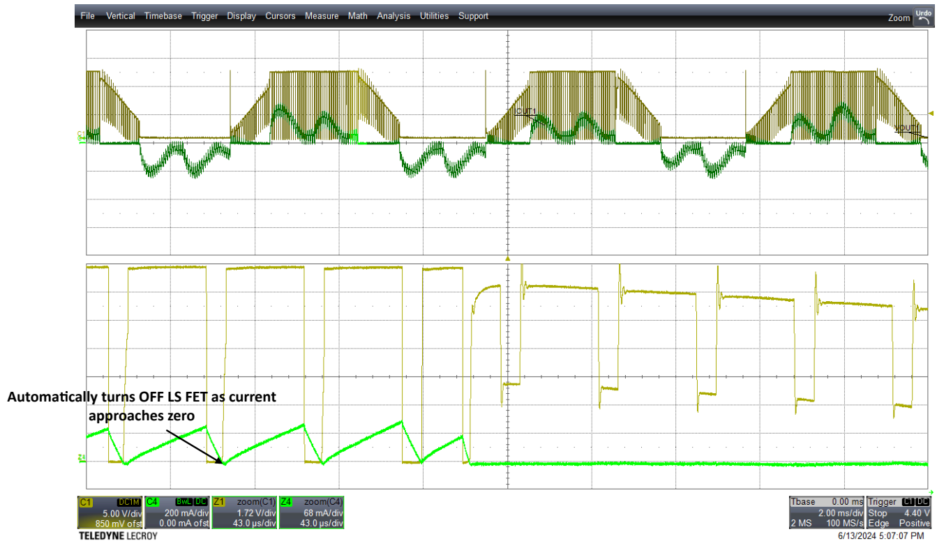
図 9-8. ASR Enabled in Synchronous Modulation
