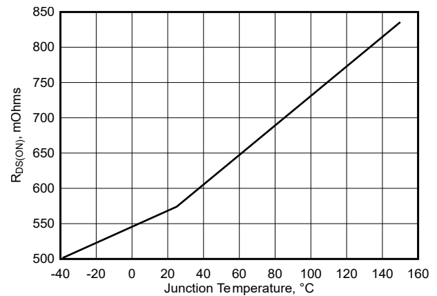
図 6-3. R_{DS(ON)} (high and low side combined) for MOSFETs over temperature
