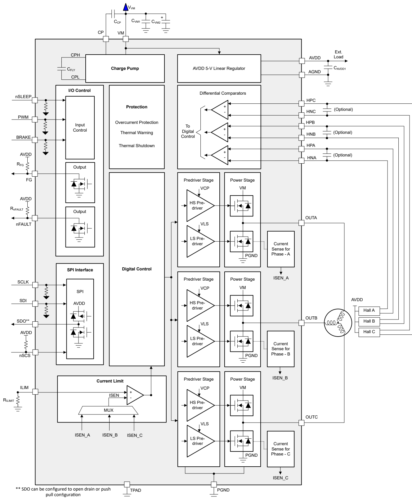
7-1. MCT8314ZS Block Diagram
