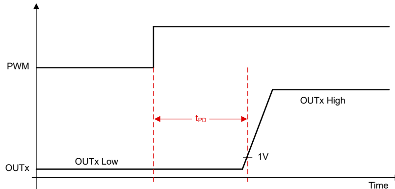
図 7-13. Propagation Delay Timing
