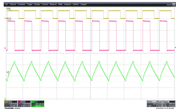
図 9-14. Driver PWM Operation with Current Limit
