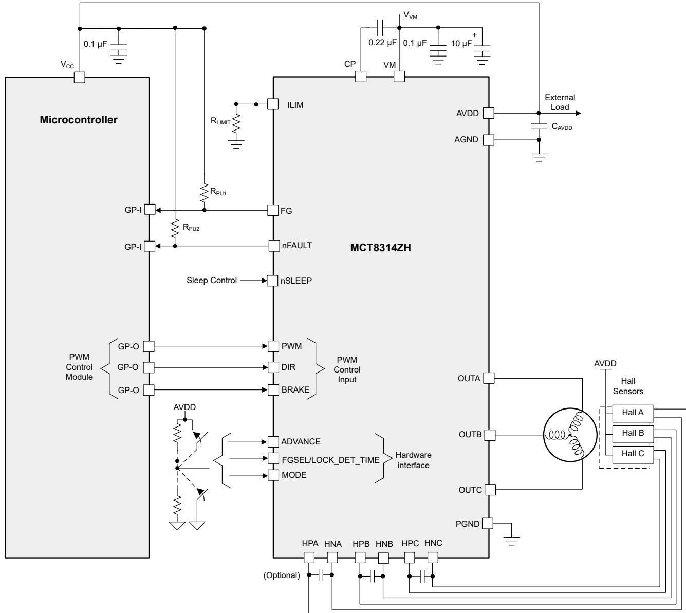
図 9-2. Primary Application Schematics for MCT8314ZH (Hardware variant)
