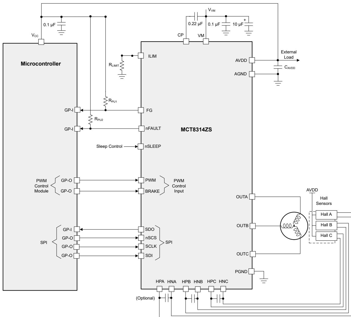
図 9-1. Primary Application Schematics for MCT8314ZS (SPI variant)
