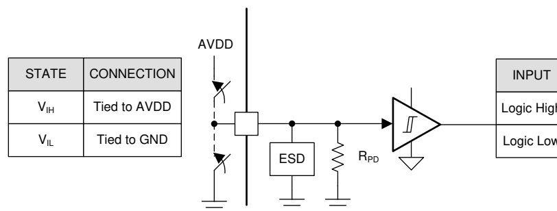
図 7-14. Logic-Level Input Pin Structure
