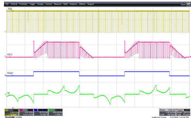
図 9-12. Driver PWM Operation with FGOUT
