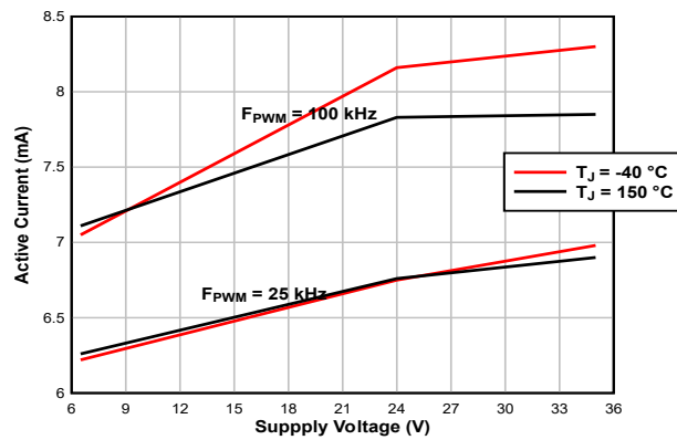
図 6-2. Supply current over supply voltage
