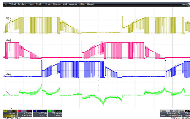
図 9-11. Driver PWM Operation
