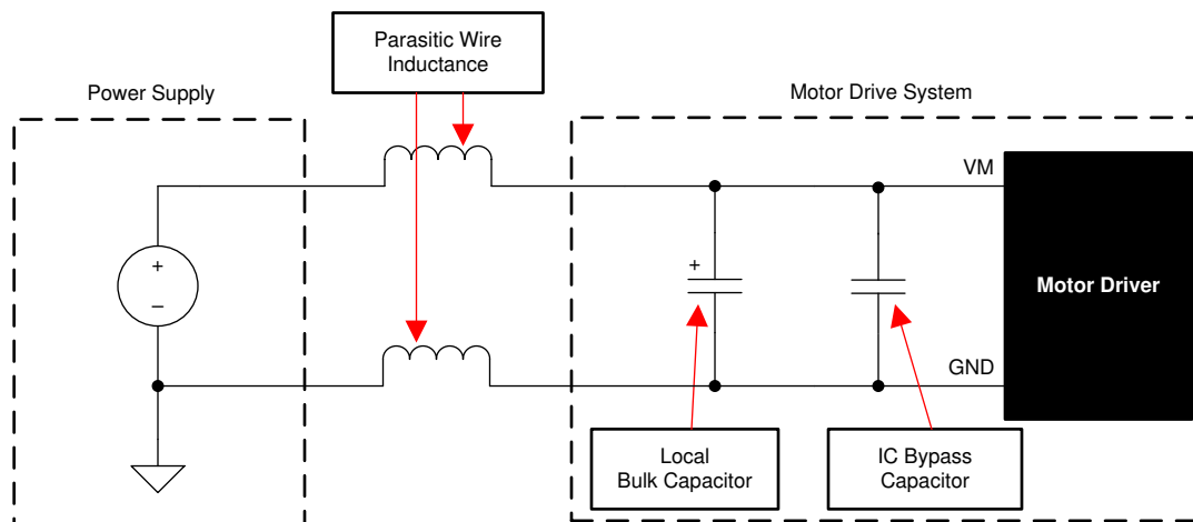
图 9-15. Example Setup of Motor Drive System With External Power Supply
