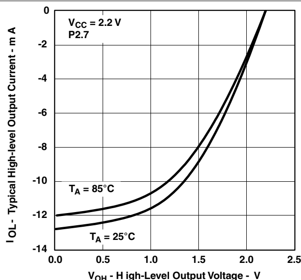
FIG 8-4. Typical High-Level Output Current vs Typical High-Level Output Current
