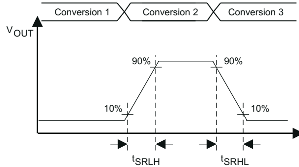
FIG 8-26. Slew Rate Testing
