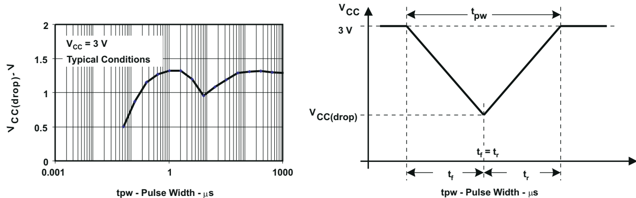
FIG 8-12. V_{CC(drop)} Level With a Triangle Voltage Drop to Generate a POR or BOR Signal
