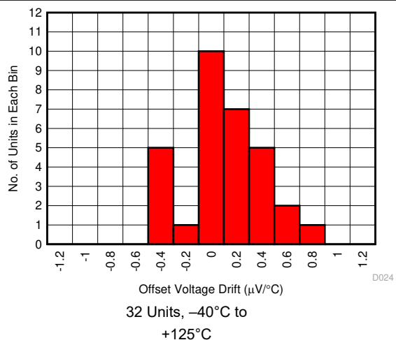
7-24. Input Offset Drift Distribution
