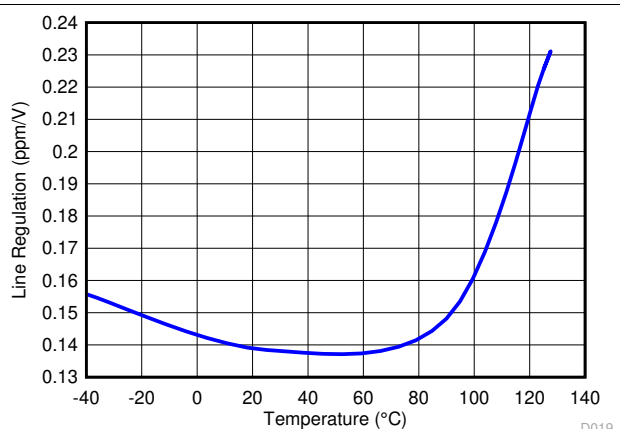
7-6. Line Regulation
