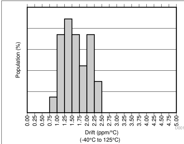
7-1. Temperature Drift
