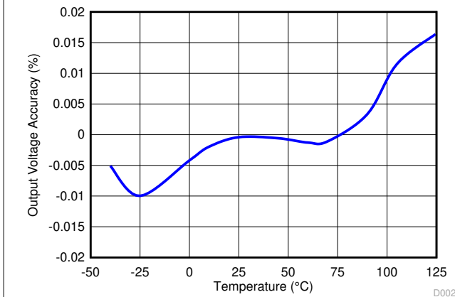
7-3. Output Voltage Accuracy vs Temperature
