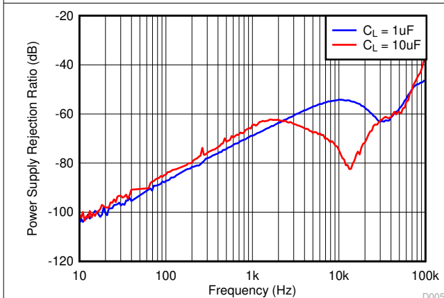
7-5. Power-Supply Rejection Ratio vs Frequency
