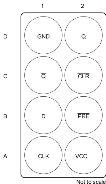
✎ 5-2. YZP Package 8-Pin DSBGA Bottom View
