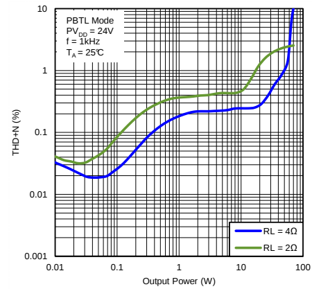
Figure 36. Total Harmonic Distortion + Noise vs Output Power (PBTL Mode)
