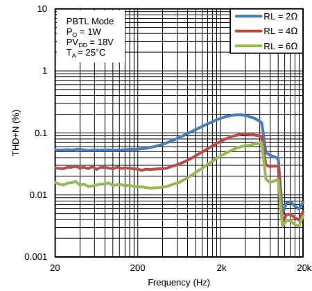
Figure 38. Total Harmonic Distortion + Noise vs Frequency (PBTL Mode)
