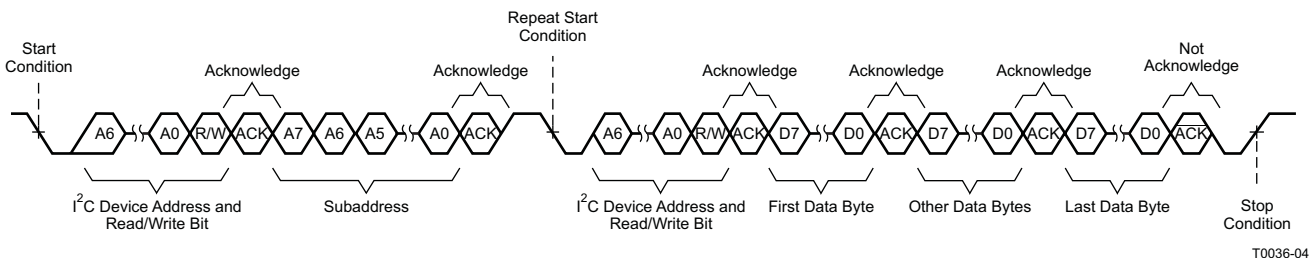
FIG 54. Multiple-Byte Read Transfer
