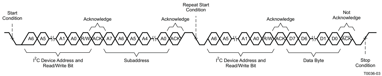
FIG 53. Single-Byte Read Transfer
