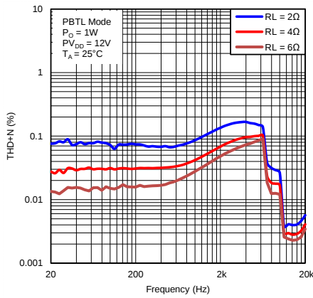
Figure 37. Total Harmonic Distortion + Noise vs Frequency (PBTL Mode)
