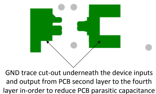
10-13. Ground Trace Cutout Beneath the Device Inputs and Output
