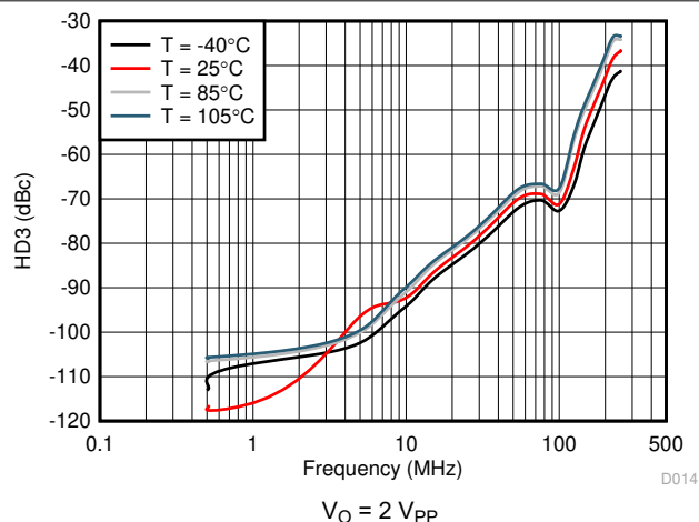
8-16. HD3 vs Frequency Across Temperature
