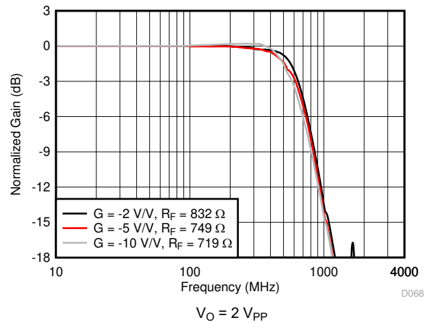
8-43. Inverting Small-Signal Frequency Response
