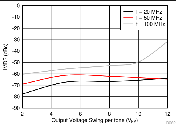
8-20. IMD3 vs Output Voltage Swing
