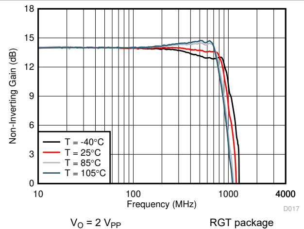
8-6. Frequency Response vs Temperature
