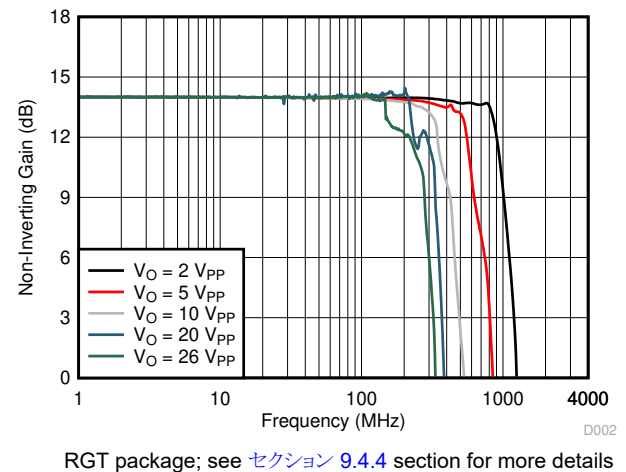
8-4. Frequency Response vs Output Swing
