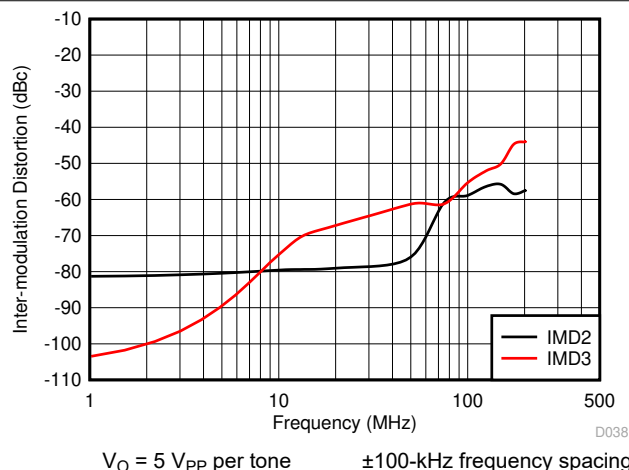
8-18. Intermodulation Distortion vs Frequency
