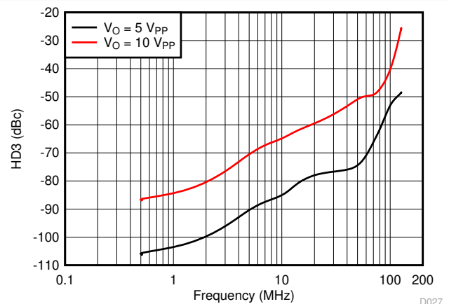
8-47. HD3 vs Frequency Across Output Swing
