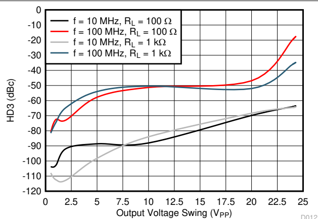
8-14. HD3 vs Output Swing
