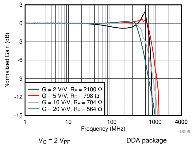
8-2. Noninverting Small-Signal Frequency Response
