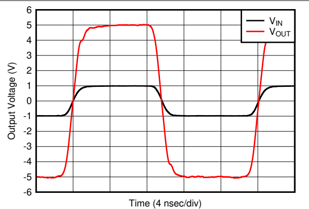
8-23. G = 5 V/V Pulse Response
