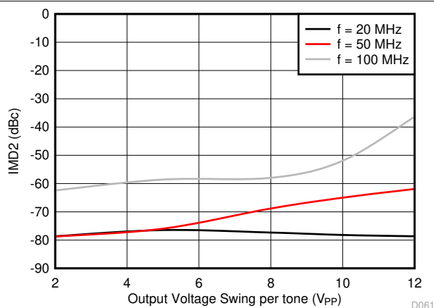
8-19. IMD2 vs Output Voltage Swing
