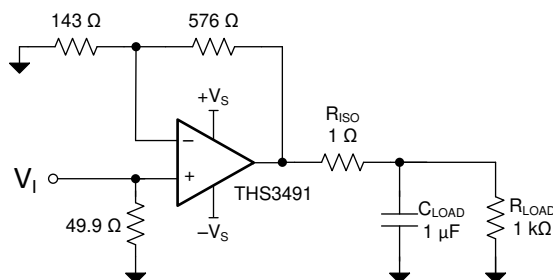
図 10-1. Driving a Large Capacitive Load Using an Output Series Isolation Resistor
