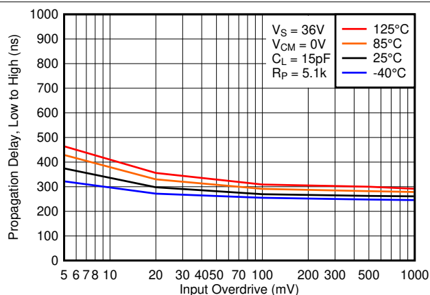
Figure 5-30. Low to High Propagation Delay vs. Input Overdrive Voltage, 36V
