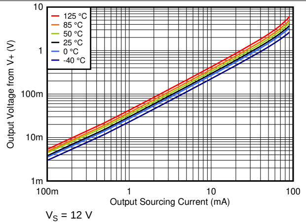
FIG 28. Output Sourcing Current vs. Output Voltage at 12V
