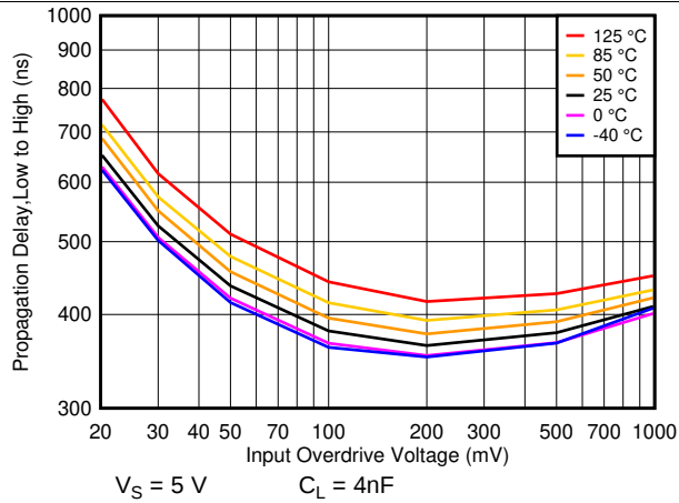
图 45. T_{PLH} Response Time vs. Overdrive at 5V
