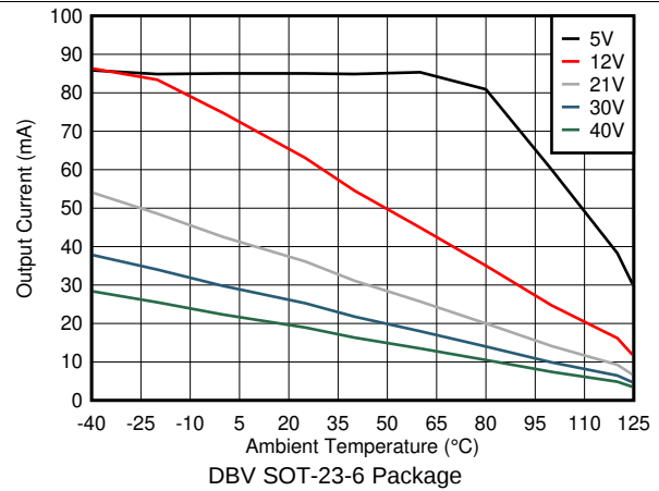
Figure 22. Maximum Output Current vs. Ambient Temperature
