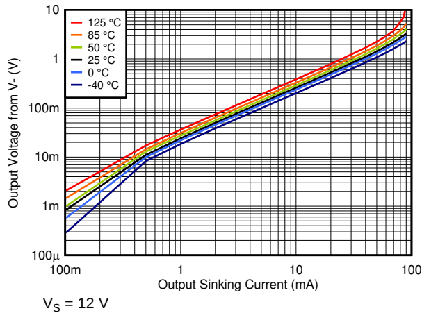
FIG 27. Output Sinking Current vs. Output Voltage at 12V
