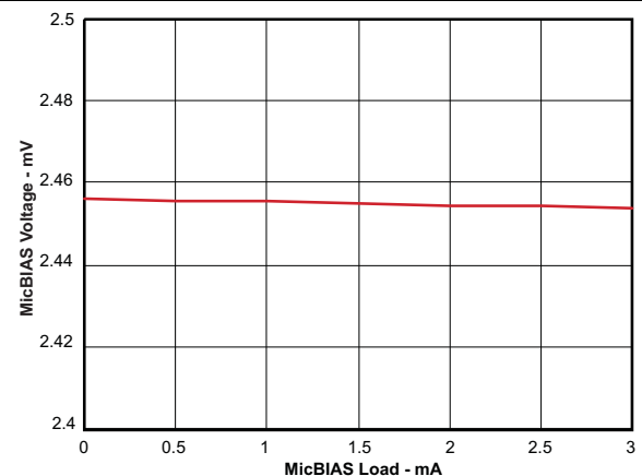
FIG 12. MICBIAS Mode 2, CM = 0.9 V, LDOIN OP Stage vs MICBIAS Load Current
