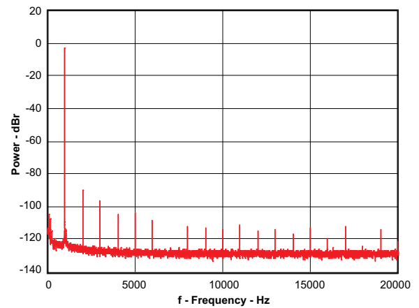
FIG 14. Analog Bypass to Headphone FFT at -3 dB Below 0.5 Vrms
