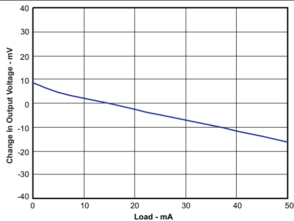
FIG 11. LDO Load Response
