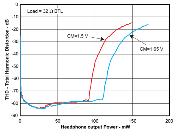
FIG 8. Total Harmonic Distortion vs Headphone Output Power
