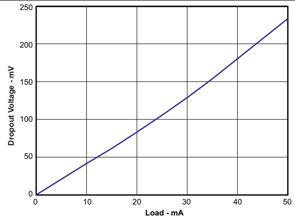
FIG 10. LDO Dropout Voltage vs Load Current
