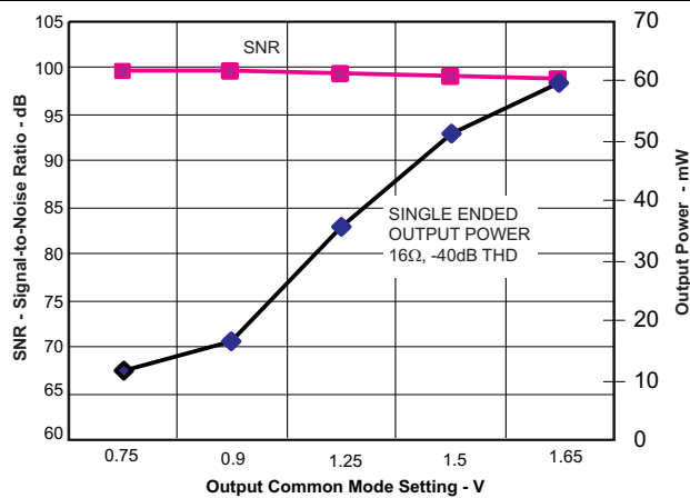
FIG 9. Headphone SNR and SE Output Power vs Output Common Mode Setting
