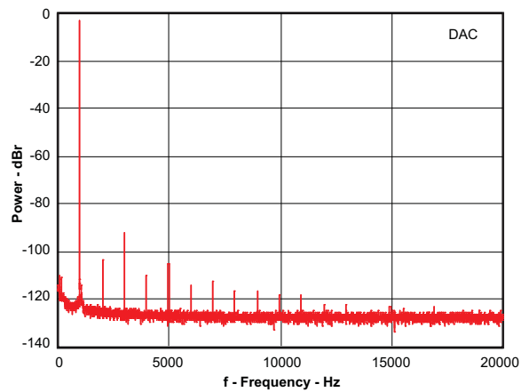
FIG 13. DAC to Headphone FFT at -3 dBFS
