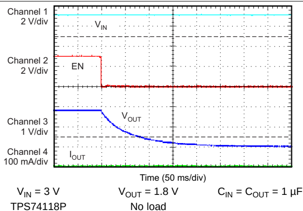
图 22. Shutdown Response With Enable
