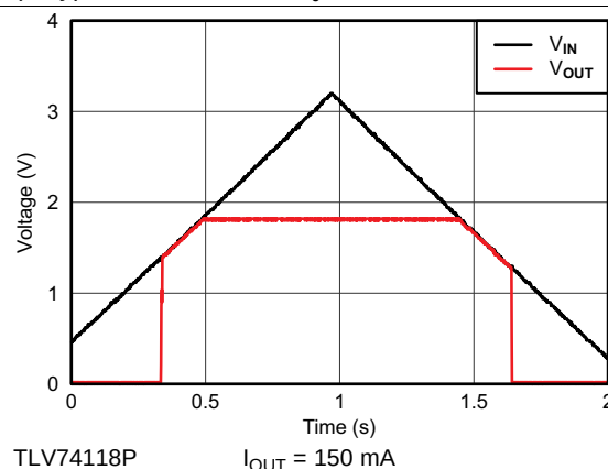
图 20. V_{IN} Power-Up and Power-Down
