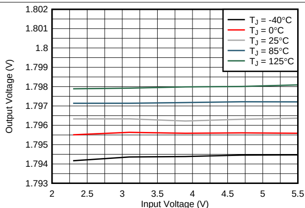
图 1. 1.8-V Line Regulation vs V_{IN} and Temperature
