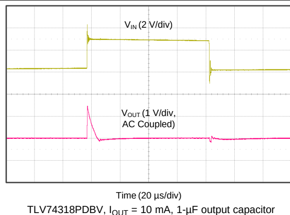
FIG 23. Line Transient
