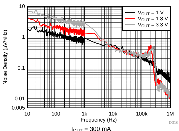
FIG 22. Output Spectral Noise Density
