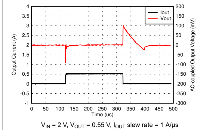
5-21. 0.55-V, 1-mA to 500-mA Load Transient
