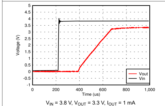
5-23. V_{IN} Power-Up
