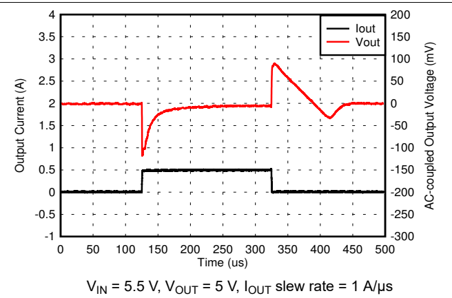
5-22. 5-V, 1-mA to 500-mA Load Transient
