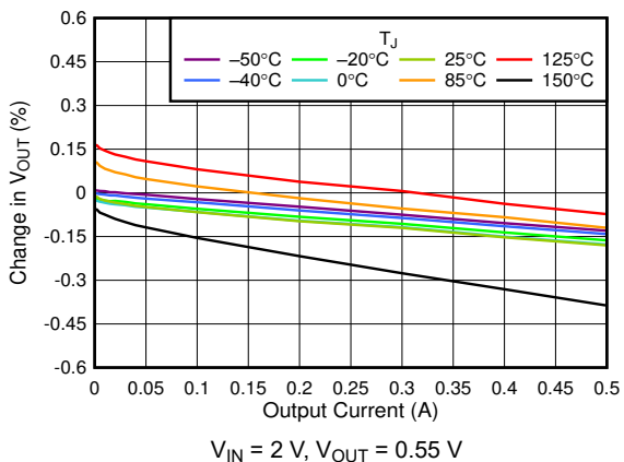
5-12. 0.55-V Load Regulation vs I_{OUT}
