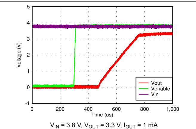
5-24. Start-Up With EN
