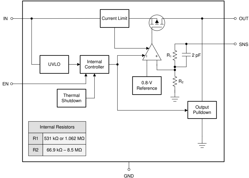
8-2. Fixed Version Block Diagram
