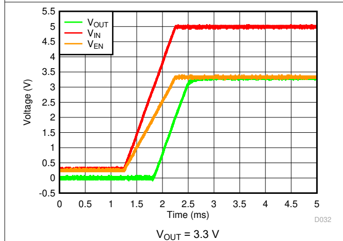
7-21. Startup With Separate V_{EN} and V_{IN}
