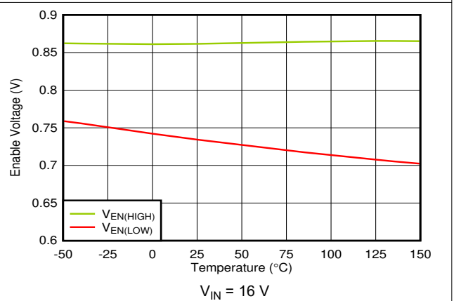
7-24. V_{EN} Thresholds vs Temperature
