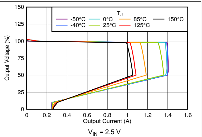
7-20. Foldback Current Limit vs Temperature
