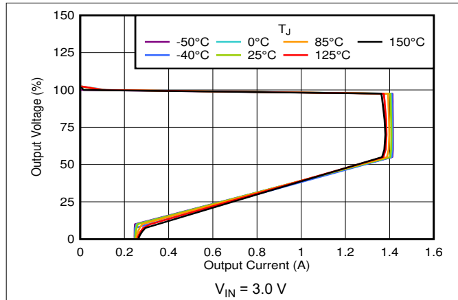
7-19. Foldback Current Limit vs Temperature
