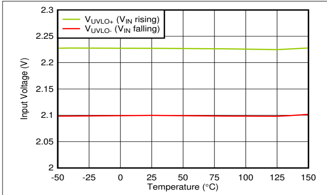
7-25. UVLO Thresholds vs Temperature
