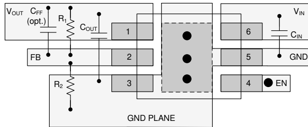
☒ 11-1. Layout Example for the Adjustable WSON Version
