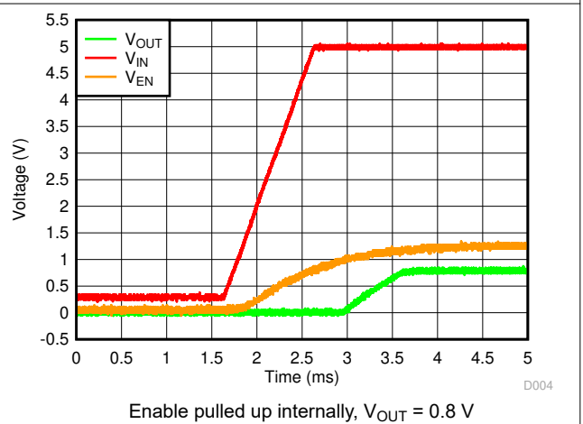
7-22. Startup With V_{EN} Floating
