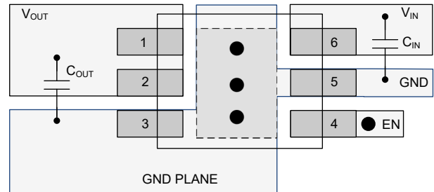
☒ 11-2. Layout Example for the Fixed WSON Version
