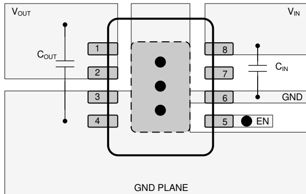
☒ 11-3. Layout Example for the Fixed HVSSOP Version
