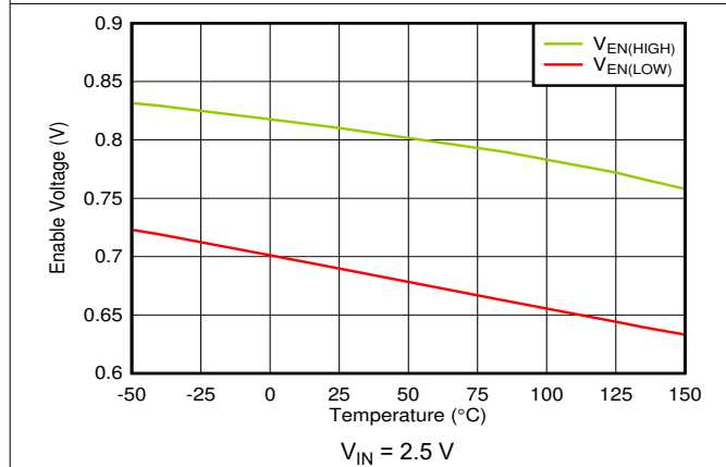
7-23. V_{EN} Thresholds vs Temperature
