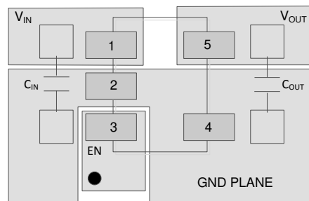
☒ 11-3. Layout Example for the Fixed HVSSOP Version
