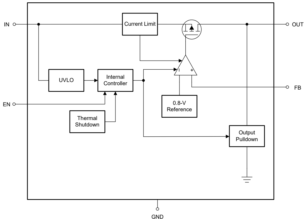
8-1. Adjustable Version Block Diagram
