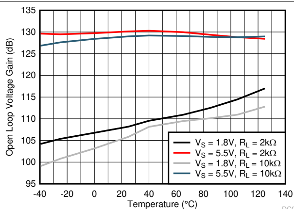
6-14. Open Loop Voltage Gain vs Temperature
