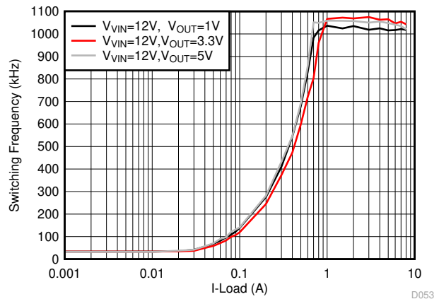
6-22. F_{sw} Load Regulation, OOA-mode, F_{sw} = 1 MHz
