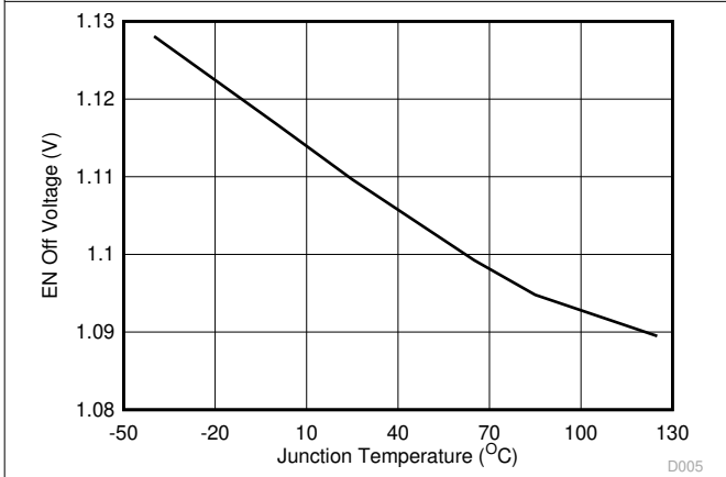
6-5. Enable Off Voltage vs Junction Temperature
