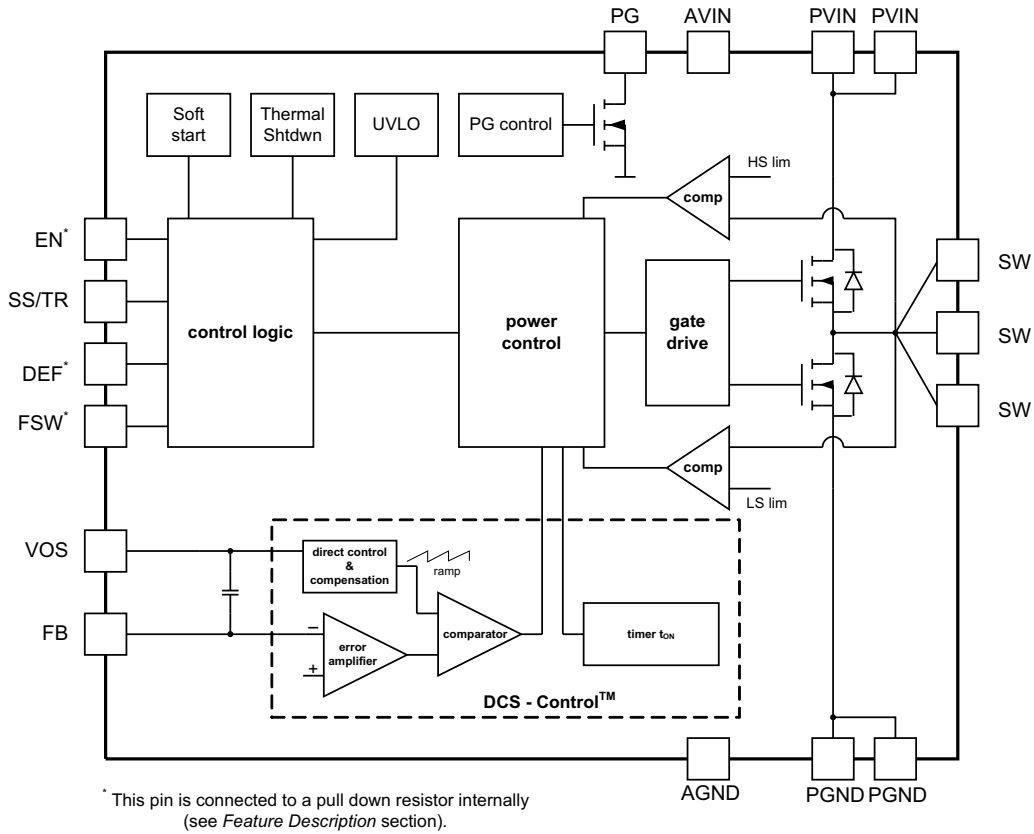
8-1. TPS62130 and TPS62130A (Adjustable Output Voltage)
