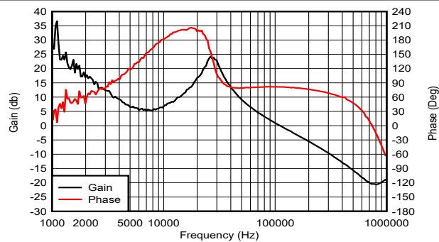
Figure 9-81. Bode Plot
