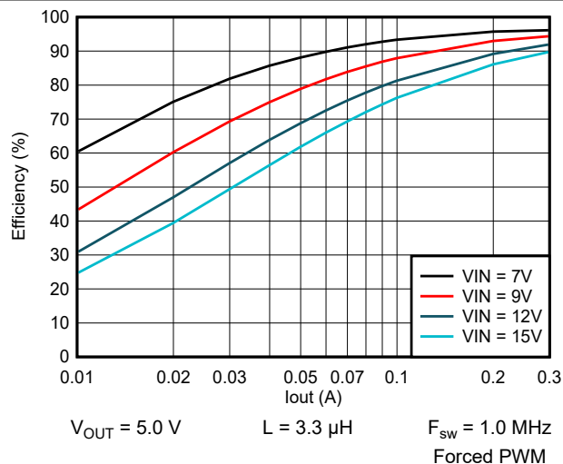
Figure 9-9. Efficiency vs Output Current
