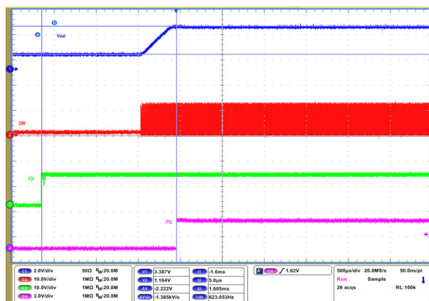
FIG 9-62. Start-Up Timing
