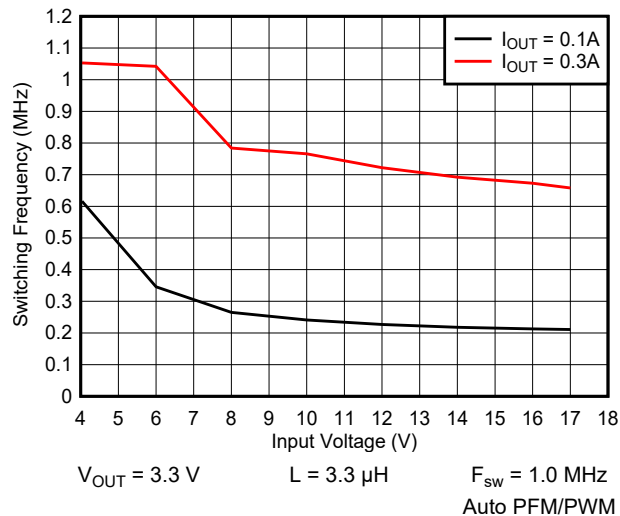
Figure 9-22. Switching Frequency vs Input Voltage
