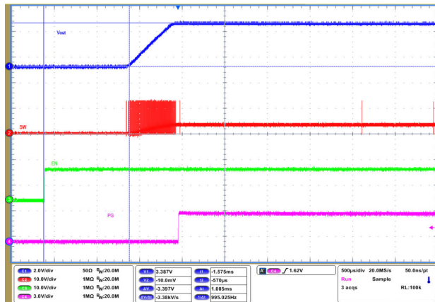
FIG 9-62. Start-Up Timing
