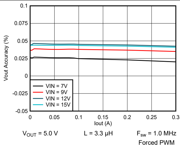
Figure 9-13. Output Voltage vs Output Current
