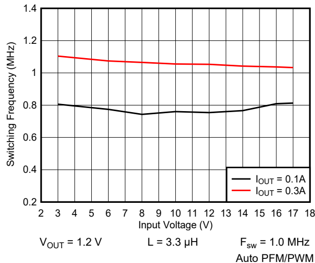
9-46. Switching Frequency vs Input Voltage
