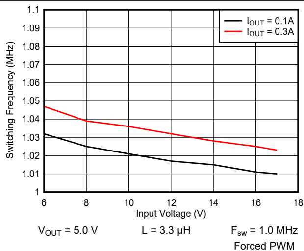
Figure 9-11. Switching Frequency vs Input Voltage
