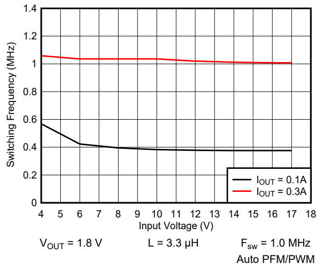
9-34. Switching Frequency vs Input Voltage
