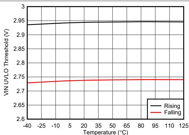
图 7-16. V_{IN} UVLO Thresholds vs Temperature
