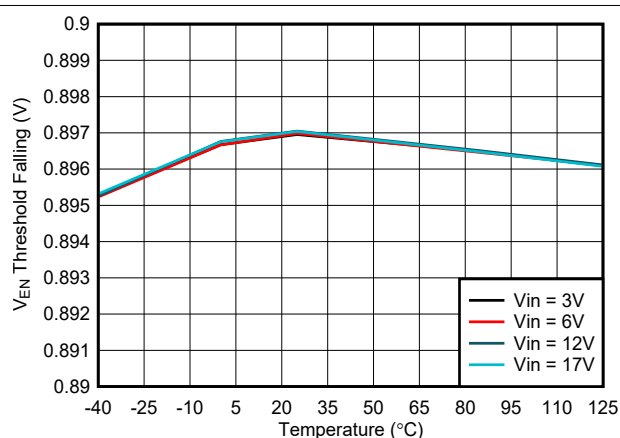
图 7-18. Precision Enable Threshold vs Temperature
