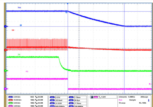
FIG 9-65. Shutdown Timing with Output Discharge Enabled
