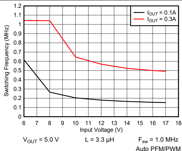
Figure 9-10. Switching Frequency vs Input Voltage
