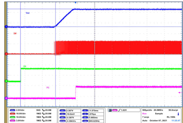
FIG 9-63. Start-Up Timing
