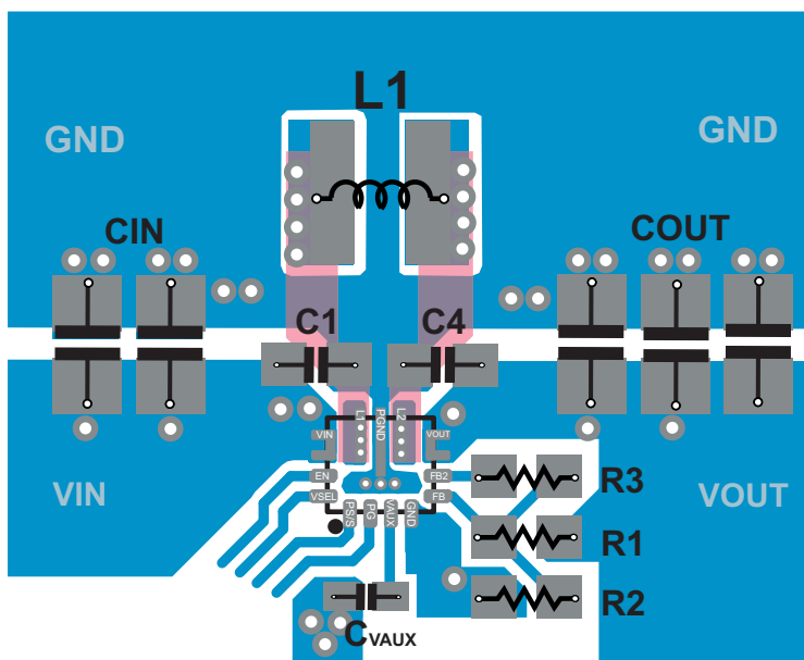
Figure 51. EVM Layout
