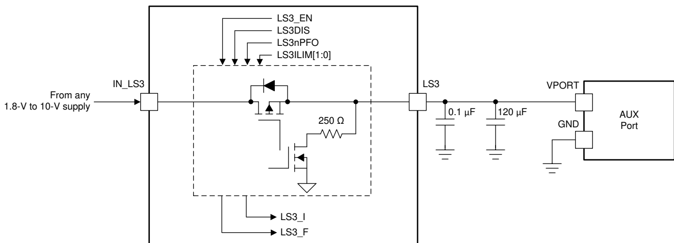
8-13. Typical Application of Load Switch 3
