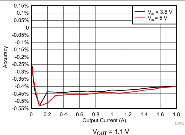
7-2. DCDC2 Accuracy
