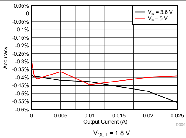
7-6. DCDC6 Accuracy
