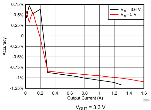
7-4. DCDC4 Accuracy
