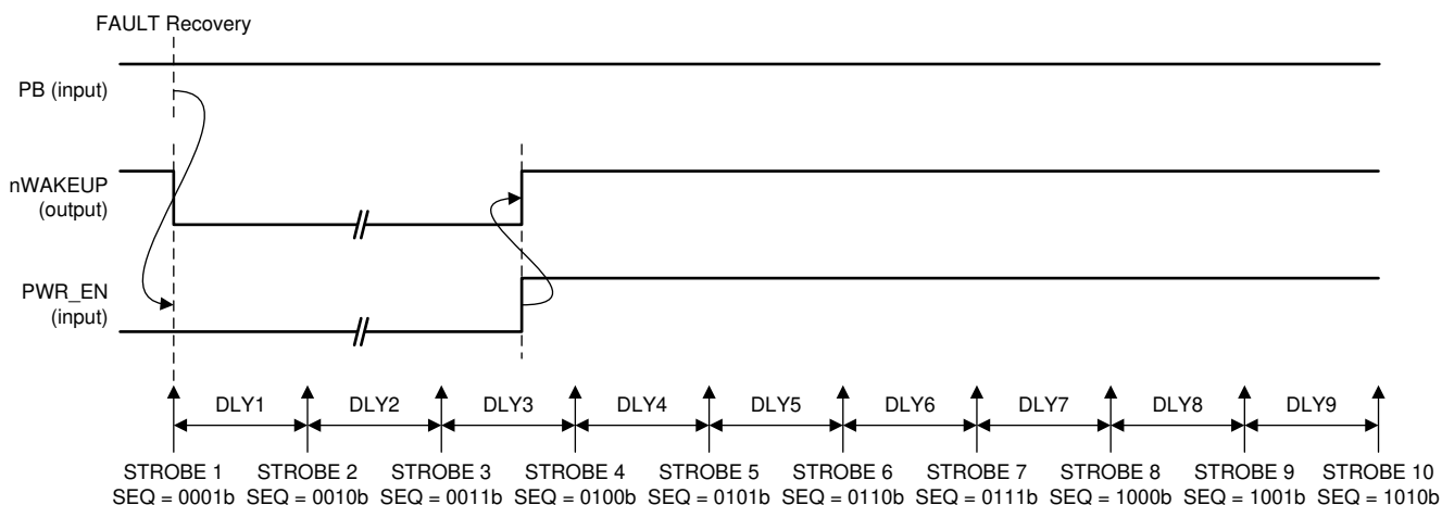
8-3. Power-Up Sequences from RECOVERY State
