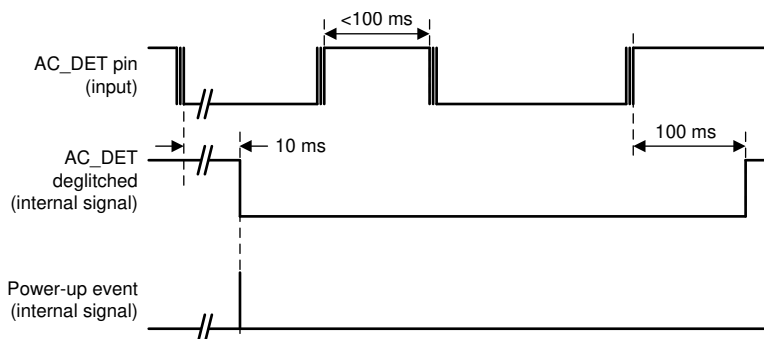
FIG 7-21. AC_DET Input Deglitch and Power-Up Timing (Portable Systems)
