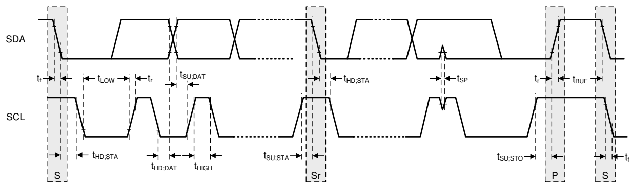
FIG 7-26. I 2 C Protocol and Transmission Timing I 2 C Data Transmission Timing
