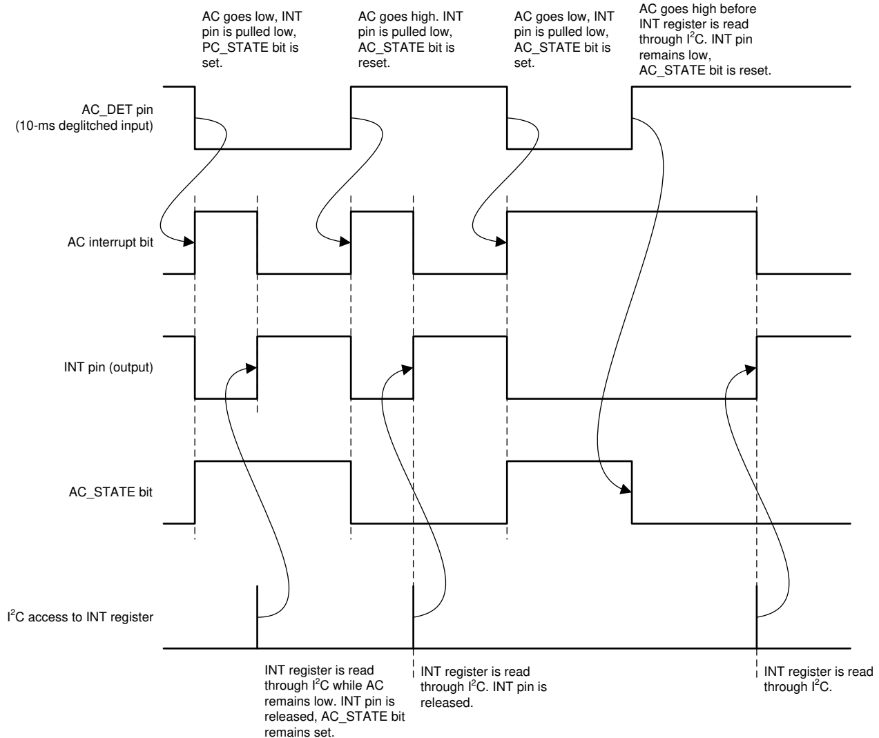
7-22. AC_STATE Pin
