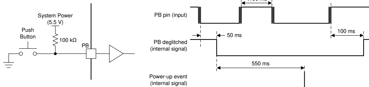
FIG 7-18. Left: Typical PB Input Circuit Right: Push-Button Input (PB) Deglitch and Power-Up Timing
