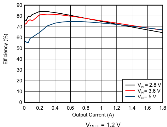
8-5. DCDC3 Efficiency
