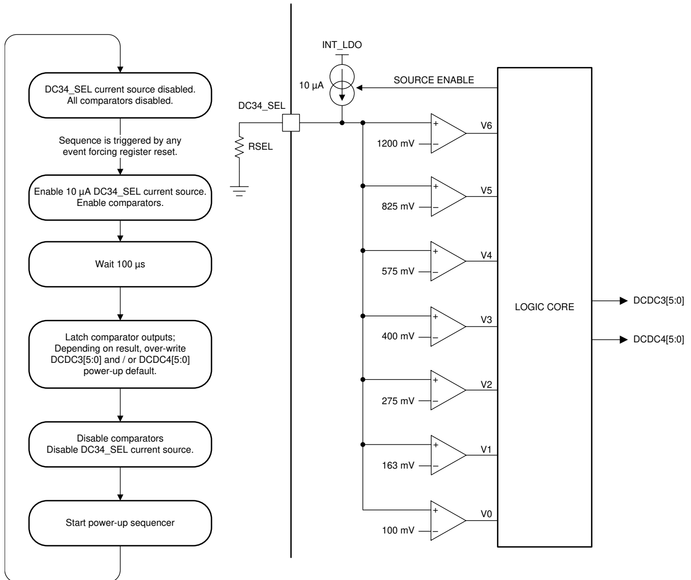
图 7-15. Left: Flow Chart for Selecting DCDC Power-Up Default Voltage Right: Comparator Circuit
