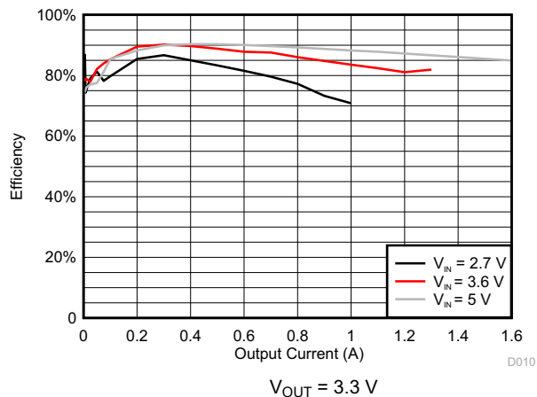
8-7. DCDC4 Efficiency
