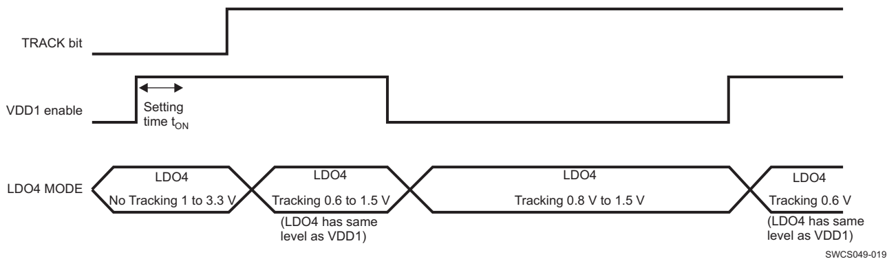
FIG 6-3. Tracking LDO
