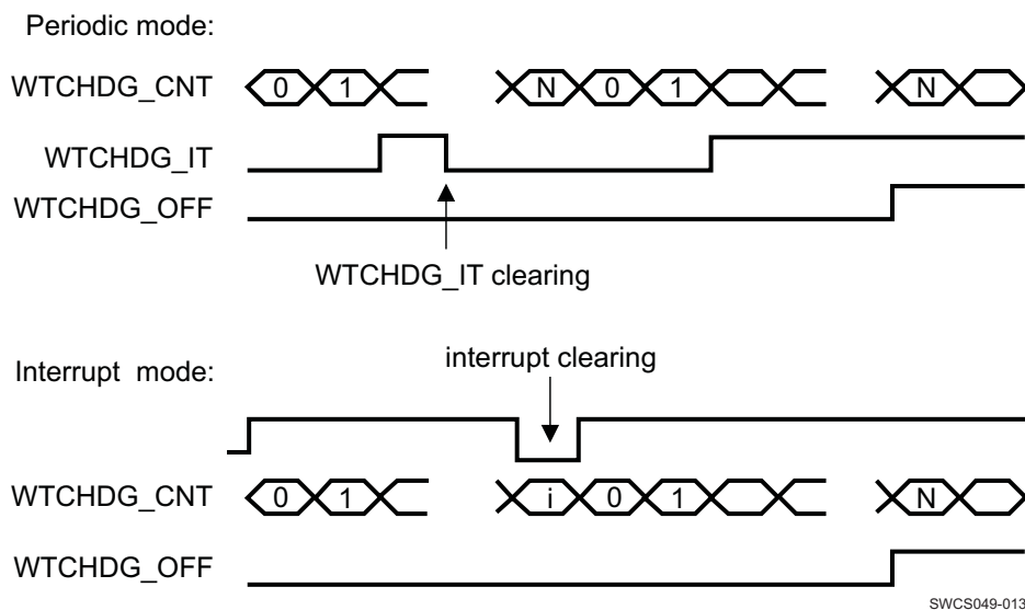
FIG 6-2. Watchdog Signals
