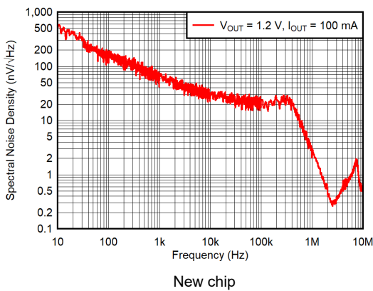
5-21. Noise Spectral Density
