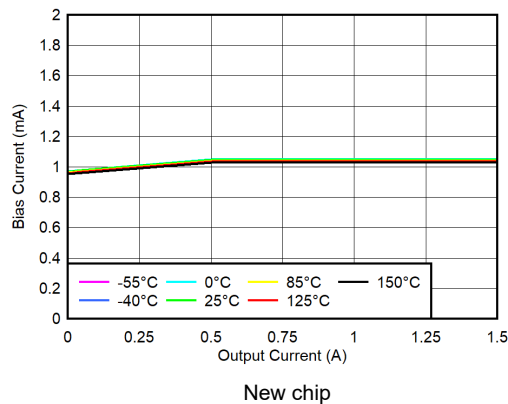
5-23. BIAS Pin Current vs Output Current and Temperature (T J )
