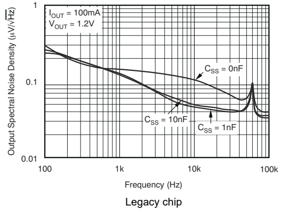
5-20. Noise Spectral Density
