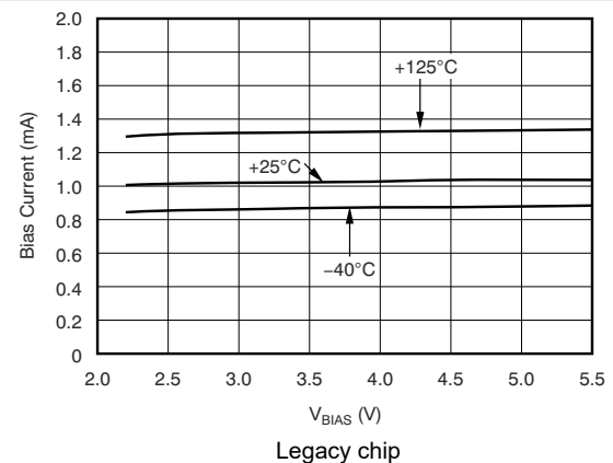
5-24. BIAS Pin Current vs V BIAS and Temperature (T J )
