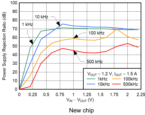
5-19. V IN PSRR vs (V IN - V OUT )
