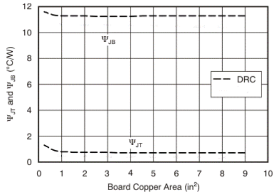
☒ 7-5. \Psi_{JT} and \Psi_{JB} vs Board Size
