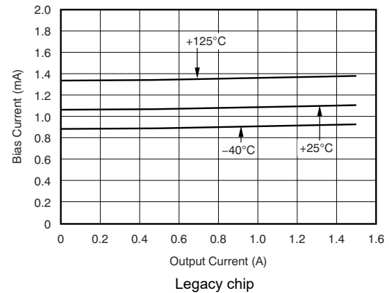
5-22. BIAS Pin Current vs Output Current and Temperature (T J )
