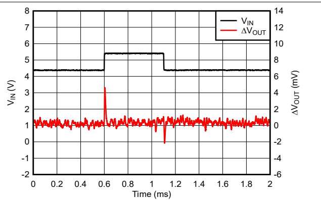
7-11. TPS76933 Line Transient Response (New Chip)
