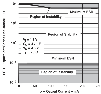
5-52. Typical Region of Stability ESR vs Output Current (Legacy Chip)
