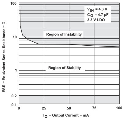
5-46. TPS76933 Typical Regions of Stability ESR vs Output Current (Legacy Chip)
