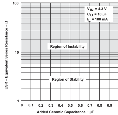
5-47. TPS76933 Typical Regions of Stability ESR vs Added Ceramic Capacitance (Legacy Chip)
