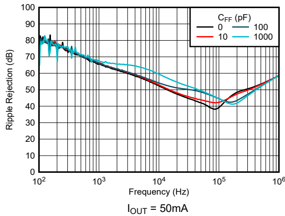
5-33. TPS76901 Ripple Rejection vs Feed-Forward Capacitor (New Chip)
