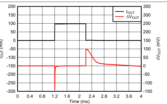
7-13. TPS76933 Load Transient Response (Legacy Chip)
