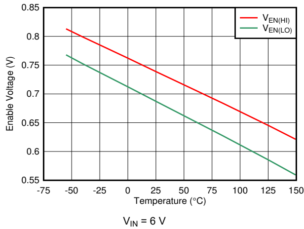
6-13. V_{EN(HI)} and V_{EN(LO)} Threshold vs Temperature
