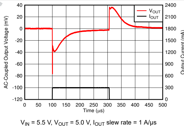
6-18. I_{OUT} Transient From 1 mA to 300 mA
