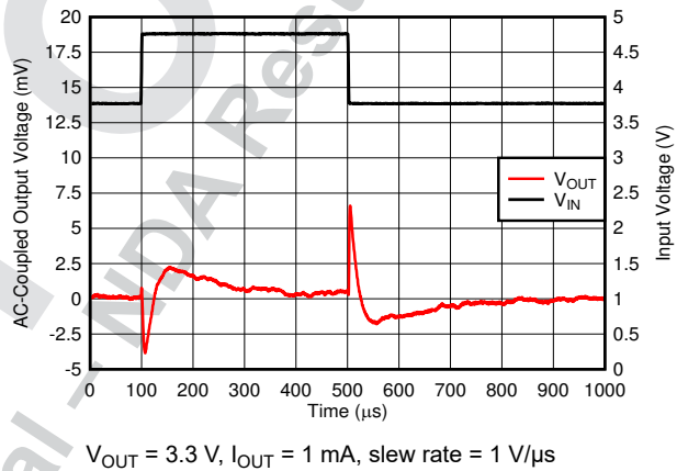
6-16. Line Transient
