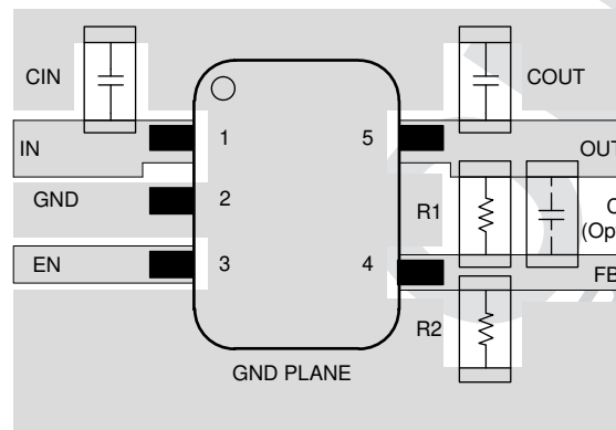
10-1. Layout Example
