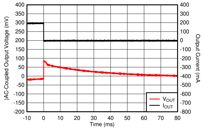
6-20. I_{OUT} Transient From 200 mA to 0 mA
