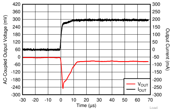
6-19. I_{OUT} Transient From 0 mA to 200 mA
