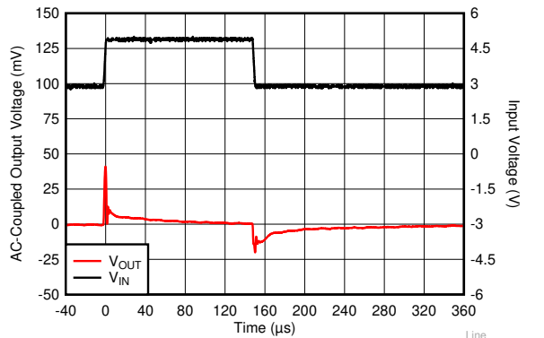
6-21. V_{IN} Transient From 2.8 V to 4.8 V
