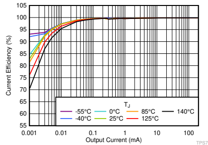
8-5. Current Efficiency vs I_{OUT} and Temperature
