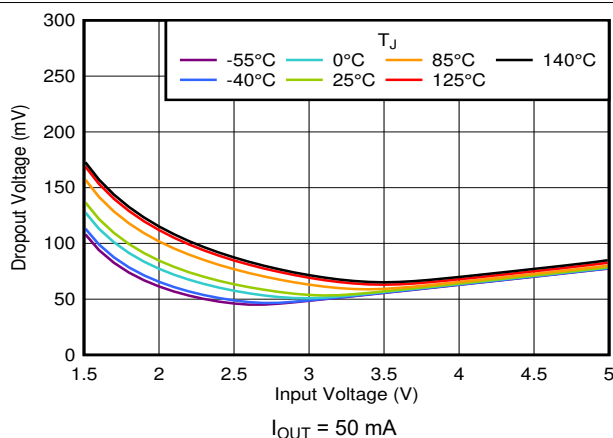
6-36. Dropout vs V_{IN} and Temperature
