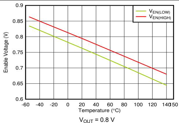
FIG 6-39. EN High and Low Threshold vs Temperature
