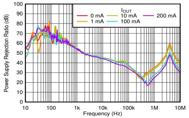
6-44. PSRR vs Frequency and I_{OUT}
