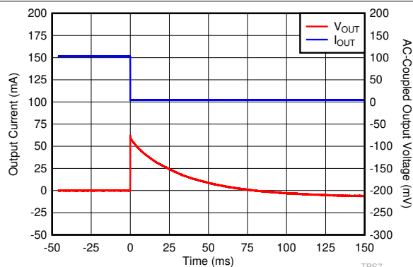
FIG 6-19. I_{OUT} Transient From 100 mA to 0 mA
