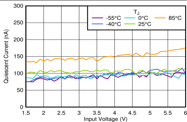
Figure 6-1. I_Q vs V_{IN} and Temperature
