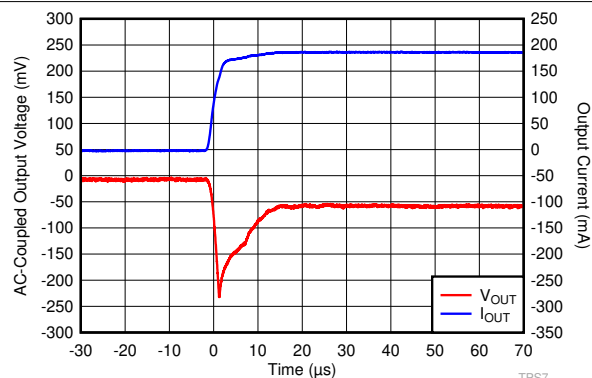
FIG 6-20. I_{OUT} Transient From 0 mA to 200 mA
