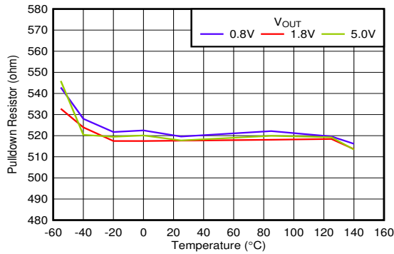
6-43. Smart Enable Pulldown Resistor vs Temperature and V_{OUT}
