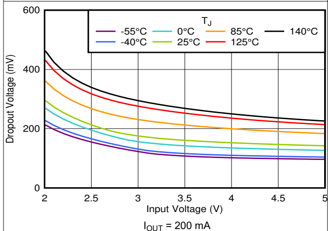
6-35. Dropout vs V_{IN} and Temperature
