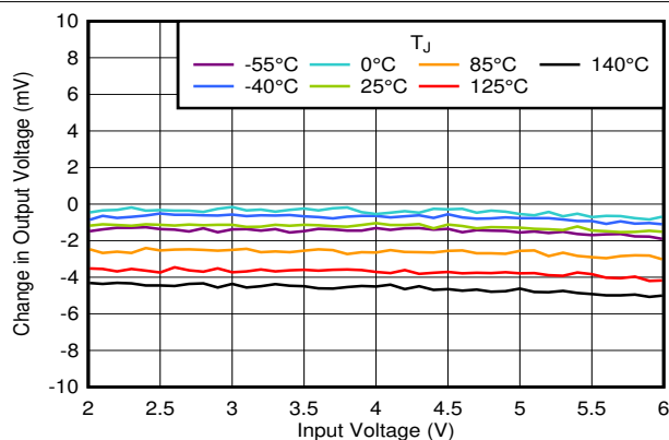
Figure 6-26. Line Regulation vs V_{IN} and Temperature
