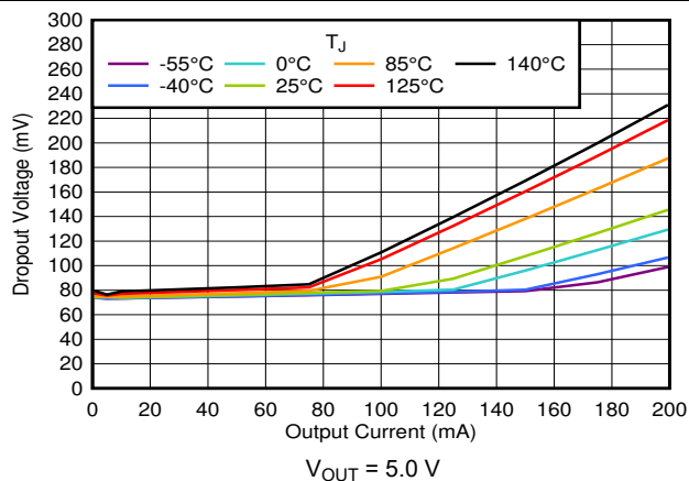
6-34. Dropout vs I_{OUT} and Temperature
