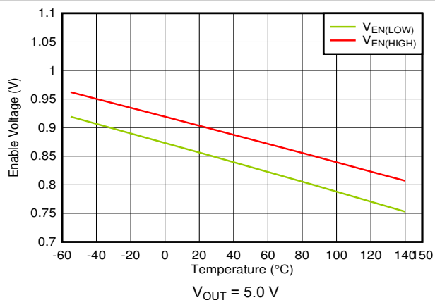
FIG 6-40. EN High and Low Threshold vs Temperature
