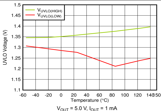
FIG 6-41. UVLO Rising and Falling Threshold vs Temperature
