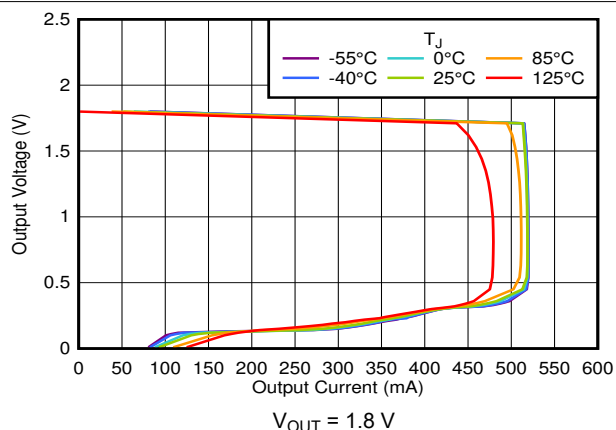
FIG 6-38. Foldback Current Limit vs I_{OUT} and Temperature
