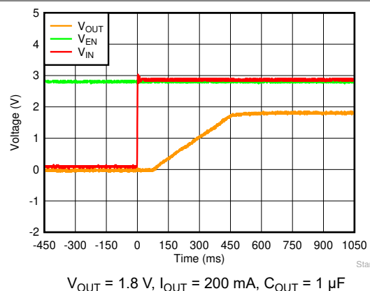
Figure 6-52. Startup With V_{EN} Before V_{IN}
