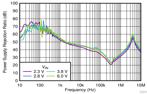
6-45. PSRR vs Frequency and V_{IN}
