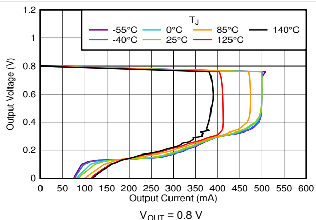
FIG 6-37. Foldback Current Limit vs I_{OUT} and Temperature
