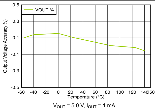
6-31. Output Accuracy vs Temperature
