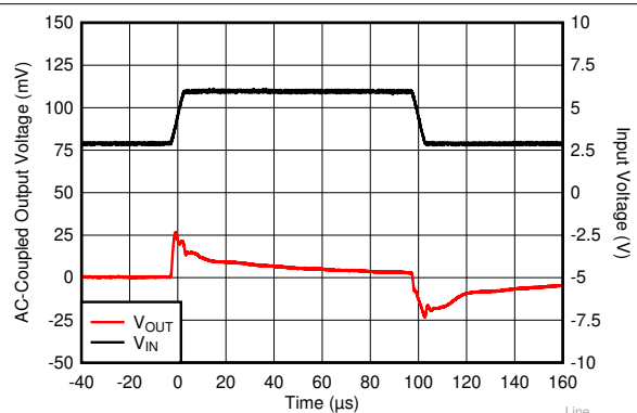
FIG 6-24. V_{IN} Transient From 2.8 V to 6.0 V
