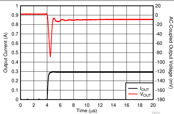
5-51. Load Transient
