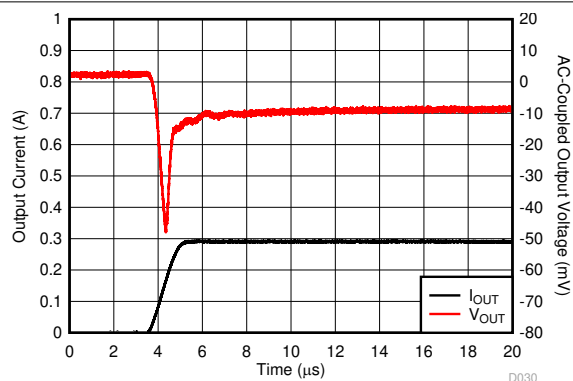
5-51. Load Transient
