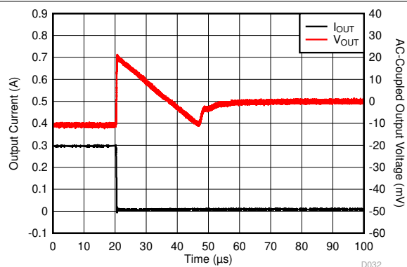
5-52. Load Transient
